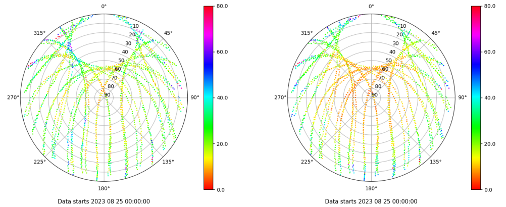
Skyplot for station SALA. Parameter M1C Data file SALA00ESP_R_2023237.xtr Skyplot for station SALA. Parameter M2P Data file SALA00ESP_R_2023237.xtr
