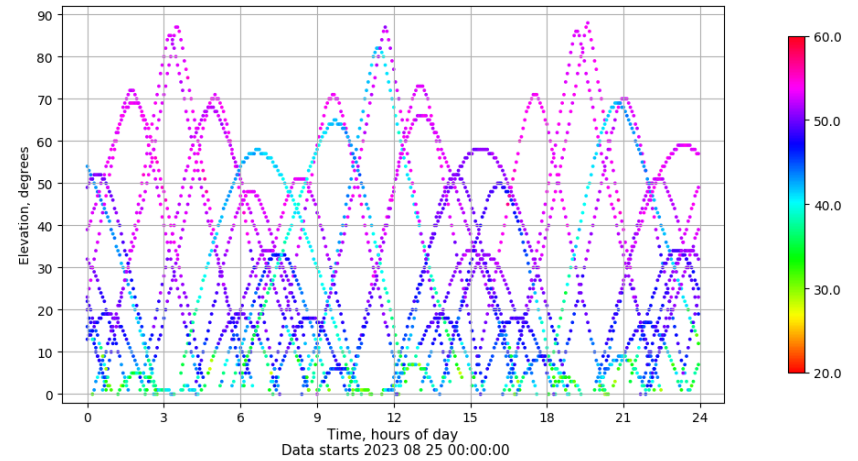
Time-elevation plot for station SALA. Signal to Noise S1C Data file SALA00ESP_R_2023237.xtr
