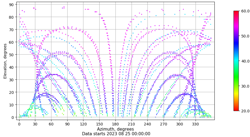
Azimuth-elevation plot for station SALA. Signal to Noise S1C Data file SALA00ESP_R_2023237.xtr
