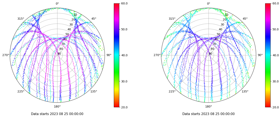
Skyplot for station SALA. Signal to Noise S1C Data file SALA00ESP_R_2023237.xtr Skyplot for station SALA. Signal to Noise S2P Data file SALA00ESP_R_2023237.xtr
