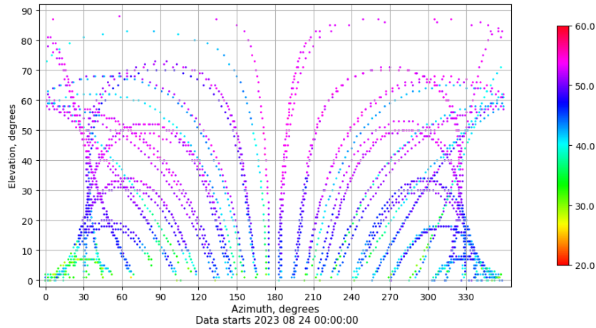
Azimuth-elevation plot for station SALA. Signal to Noise S1C Data file SALA00ESP_R_2023236.xtr
