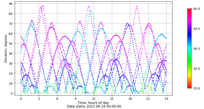
Time-elevation plot for station SALA. Signal to Noise S1C Data file SALA00ESP_R_2023236.xtr
