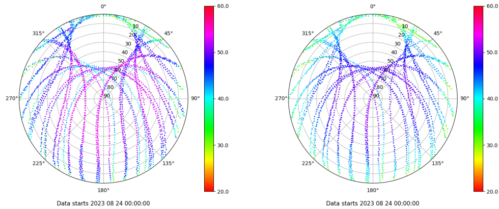
Skyplot for station SALA. Signal to Noise S1C Data file SALA00ESP_R_2023236.xtr Skyplot for station SALA. Signal to Noise S2P Data file SALA00ESP_R_2023236.xtr
