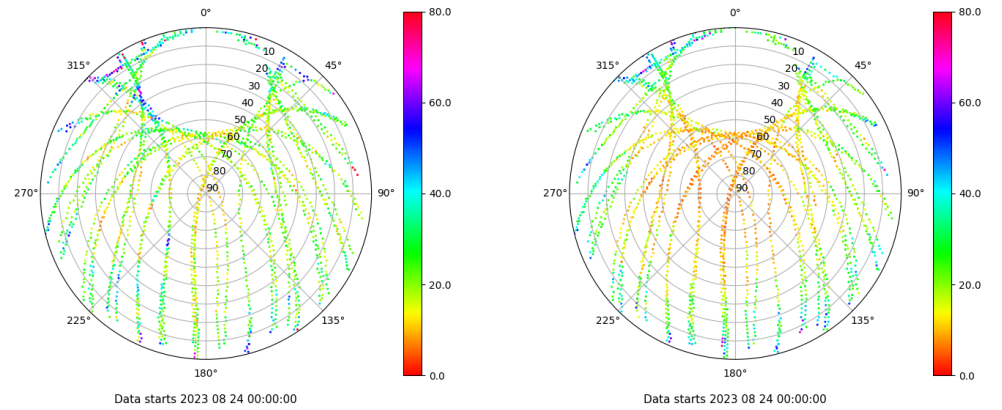
Skyplot for station SALA. Parameter M1C Data file SALA00ESP_R_2023236.xtr Skyplot for station SALA. Parameter M2P Data file SALA00ESP_R_2023236.xtr
