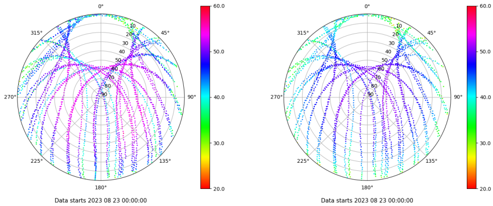
Skyplot for station SALA. Signal to Noise S1C Data file SALA00ESP_R_2023235.xtr Skyplot for station SALA. Signal to Noise S2P Data file SALA00ESP_R_2023235.xtr
