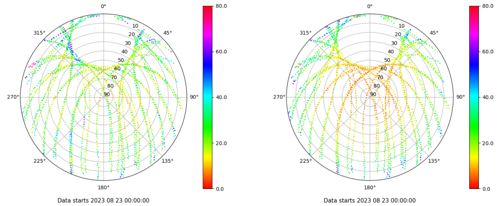
Skyplot for station SALA. Parameter M1C Data file SALA00ESP_R_2023235.xtr Skyplot for station SALA. Parameter M2P Data file SALA00ESP_R_2023235.xtr
