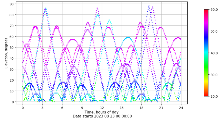
Time-elevation plot for station SALA. Signal to Noise S1C Data file SALA00ESP_R_2023235.xtr
