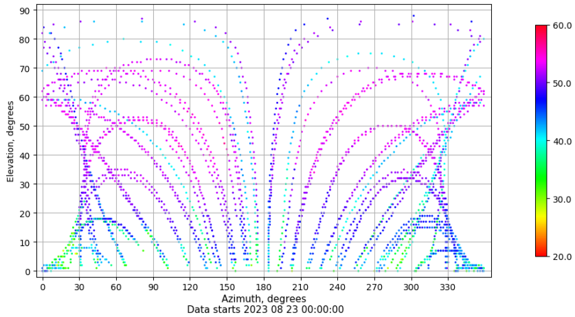
Azimuth-elevation plot for station SALA. Signal to Noise S1C Data file SALA00ESP_R_2023235.xtr
