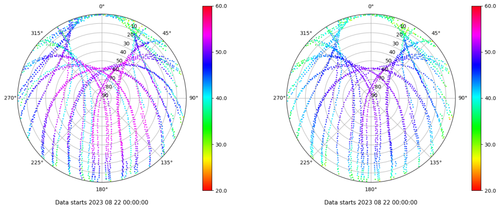
Skyplot for station SALA. Signal to Noise S1C Data file SALA00ESP_R_2023234.xtr Skyplot for station SALA. Signal to Noise S2P Data file SALA00ESP_R_2023234.xtr
