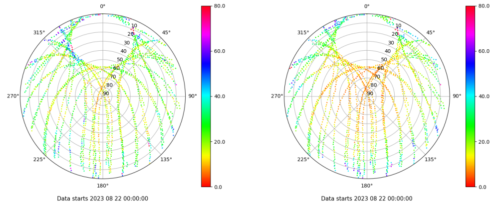
Skyplot for station SALA. Parameter M1C Data file SALA00ESP_R_2023234.xtr Skyplot for station SALA. Parameter M2P Data file SALA00ESP_R_2023234.xtr
