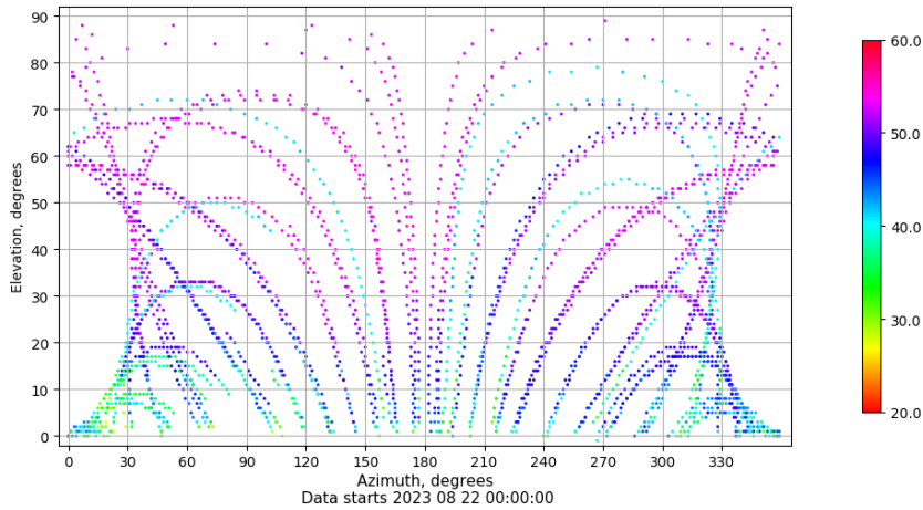
Azimuth-elevation plot for station SALA. Signal to Noise S1C Data file SALA00ESP_R_2023234.xtr
