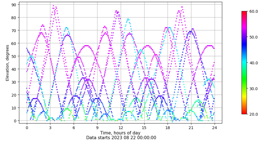
Time-elevation plot for station SALA. Signal to Noise S1C Data file SALA00ESP_R_2023234.xtr
