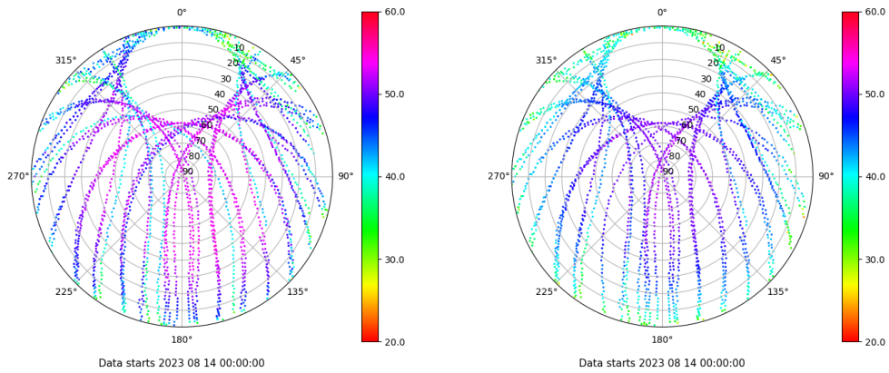
Skyplot for station SALA. Signal to Noise S1C Data file SALA00ESP_R_2023226.xtr Skyplot for station SALA. Signal to Noise S2P Data file SALA00ESP_R_2023226.xtr
