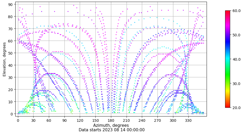
Azimuth-elevation plot for station SALA. Signal to Noise S1C Data file SALA00ESP_R_2023226.xtr
