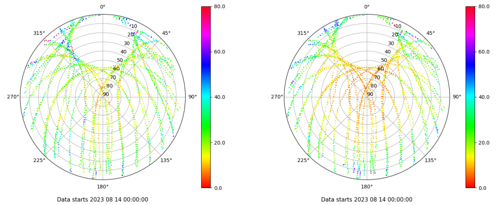
Skyplot for station SALA. Parameter M1C Data file SALA00ESP_R_2023226.xtr Skyplot for station SALA. Parameter M2P Data file SALA00ESP_R_2023226.xtr
