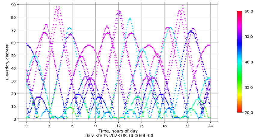
Time-elevation plot for station SALA. Signal to Noise S1C Data file SALA00ESP_R_2023226.xtr
