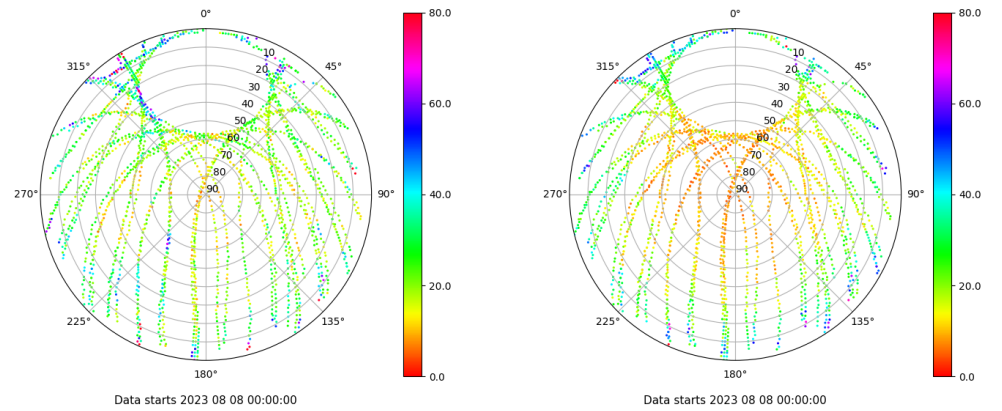
Skyplot for station SALA. Parameter M1C Data file SALA00ESP_R_2023220.xtr Skyplot for station SALA. Parameter M2P Data file SALA00ESP_R_2023220.xtr
