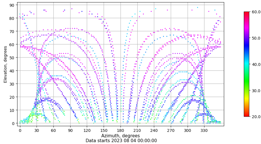
Azimuth-elevation plot for station SALA. Signal to Noise S1C Data file SALA00ESP_R_2023216.xtr
