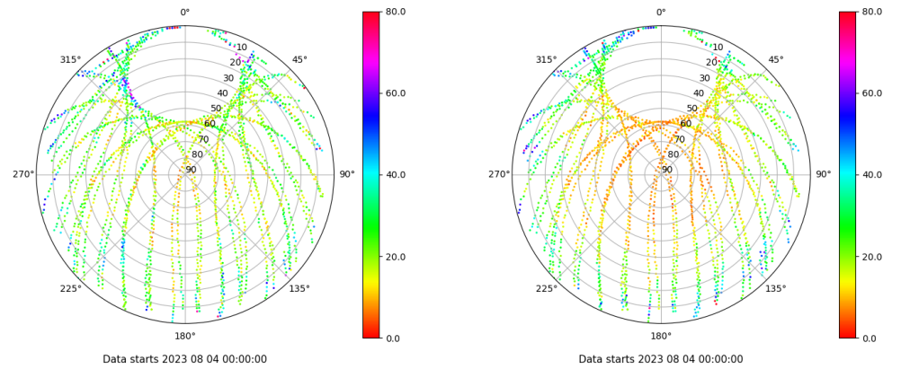
Skyplot for station SALA. Parameter M1C Data file SALA00ESP_R_2023216.xtr Skyplot for station SALA. Parameter M2P Data file SALA00ESP_R_2023216.xtr
