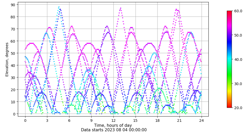
Time-elevation plot for station SALA. Signal to Noise S1C Data file SALA00ESP_R_2023216.xtr
