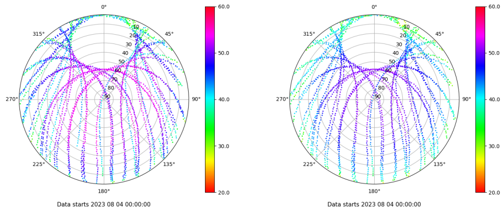
Skyplot for station SALA. Signal to Noise S1C Data file SALA00ESP_R_2023216.xtr Skyplot for station SALA. Signal to Noise S2P Data file SALA00ESP_R_2023216.xtr
