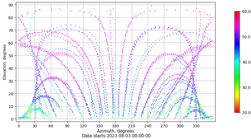
Azimuth-elevation plot for station SALA. Signal to Noise S1C Data file SALA00ESP_R_2023215.xtr
