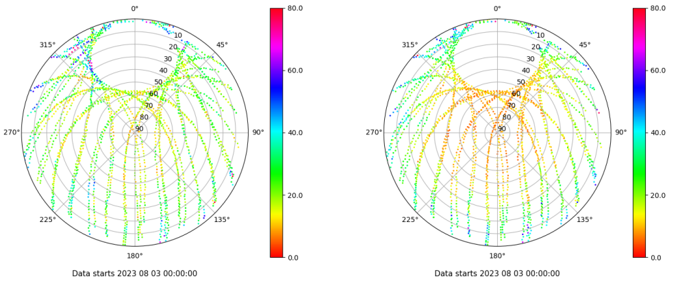
Skyplot for station SALA. Parameter M1C Data file SALA00ESP_R_2023215.xtr Skyplot for station SALA. Parameter M2P Data file SALA00ESP_R_2023215.xtr
