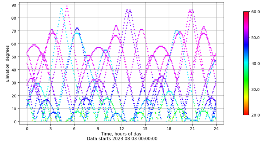
Time-elevation plot for station SALA. Signal to Noise S1C Data file SALA00ESP_R_2023215.xtr
