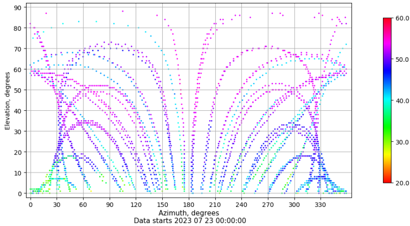
Azimuth-elevation plot for station SALA. Signal to Noise S1C Data file SALA00ESP_R_2023204.xtr
