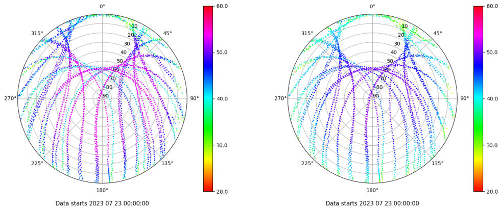
Skyplot for station SALA. Signal to Noise S1C Data file SALA00ESP_R_2023204.xtr Skyplot for station SALA. Signal to Noise S2P Data file SALA00ESP_R_2023204.xtr
