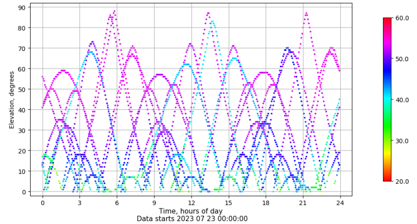
Time-elevation plot for station SALA. Signal to Noise S1C Data file SALA00ESP_R_2023204.xtr
