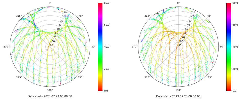
Skyplot for station SALA. Parameter M1C Data file SALA00ESP_R_2023204.xtr Skyplot for station SALA. Parameter M2P Data file SALA00ESP_R_2023204.xtr
