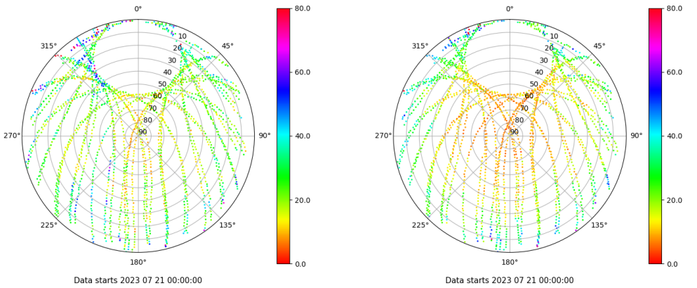
Skyplot for station SALA. Parameter M1C Data file SALA00ESP_R_2023202.xtr Skyplot for station SALA. Parameter M2P Data file SALA00ESP_R_2023202.xtr
