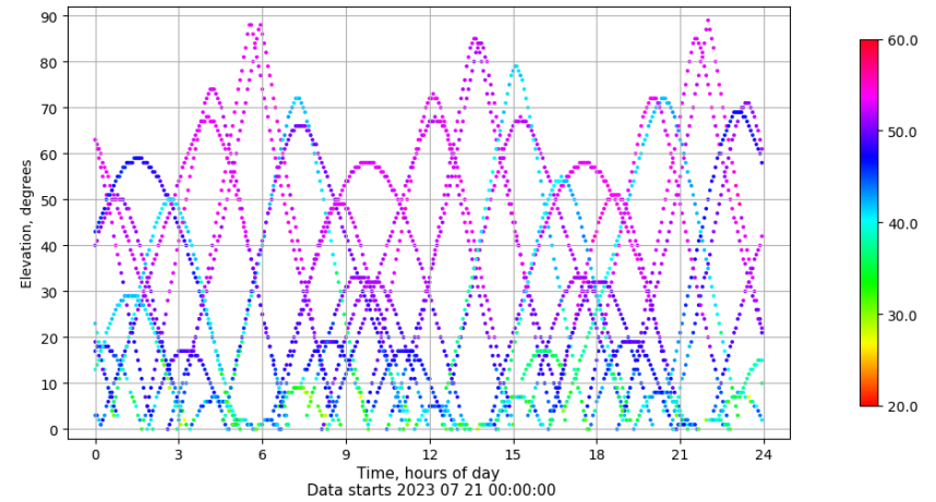
Time-elevation plot for station SALA. Signal to Noise S1C Data file SALA00ESP_R_2023202.xtr
