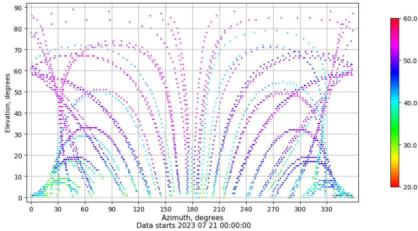
Azimuth-elevation plot for station SALA. Signal to Noise S1C Data file SALA00ESP_R_2023202.xtr
