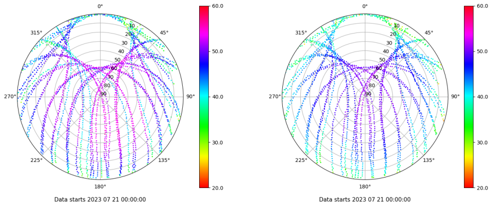
Skyplot for station SALA. Signal to Noise S1C Data file SALA00ESP_R_2023202.xtr Skyplot for station SALA. Signal to Noise S2P Data file SALA00ESP_R_2023202.xtr
