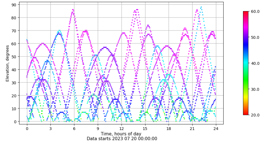
Time-elevation plot for station SALA. Signal to Noise S1C Data file SALA00ESP_R_2023201.xtr
