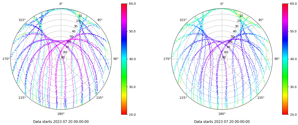
Skyplot for station SALA. Signal to Noise S1C Data file SALA00ESP_R_2023201.xtr Skyplot for station SALA. Signal to Noise S2P Data file SALA00ESP_R_2023201.xtr
