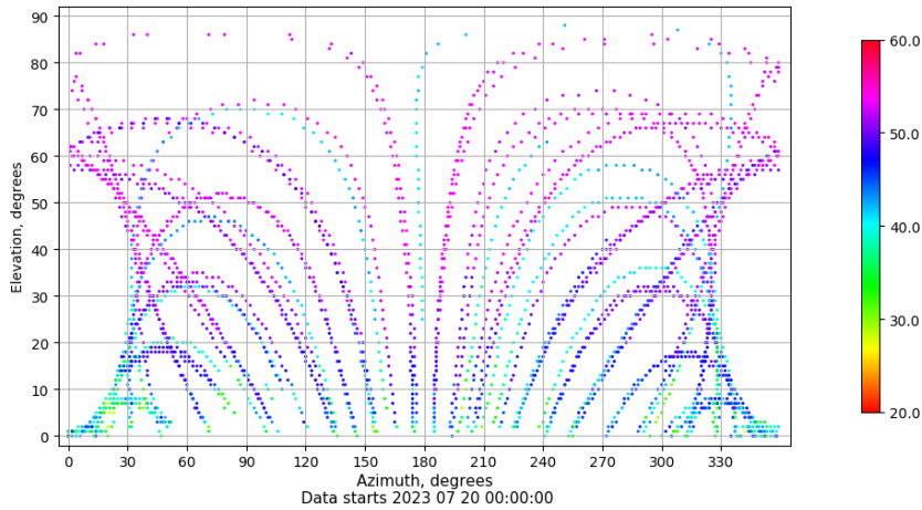
Azimuth-elevation plot for station SALA. Signal to Noise S1C Data file SALA00ESP_R_2023201.xtr
