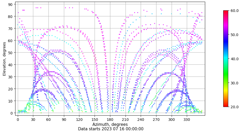
Azimuth-elevation plot for station SALA. Signal to Noise S1C Data file SALA00ESP_R_2023197.xtr
