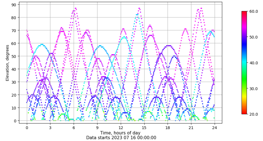
Time-elevation plot for station SALA. Signal to Noise S1C Data file SALA00ESP_R_2023197.xtr
