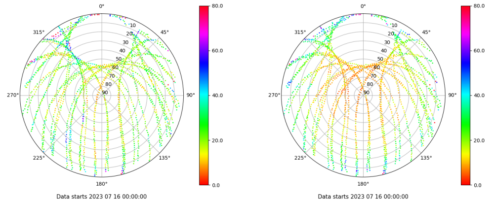
Skyplot for station SALA. Parameter M1C Data file SALA00ESP_R_2023197.xtr Skyplot for station SALA. Parameter M2P Data file SALA00ESP_R_2023197.xtr
