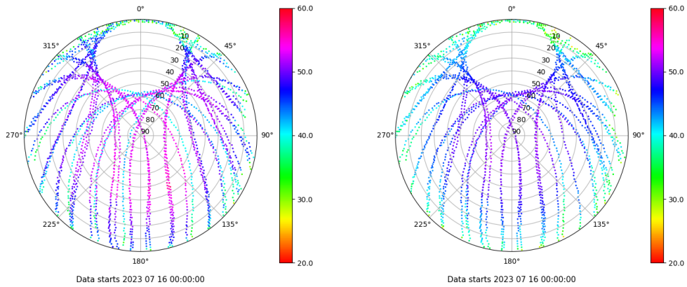
Skyplot for station SALA. Signal to Noise S1C Data file SALA00ESP_R_2023197.xtr Skyplot for station SALA. Signal to Noise S2P Data file SALA00ESP_R_2023197.xtr
