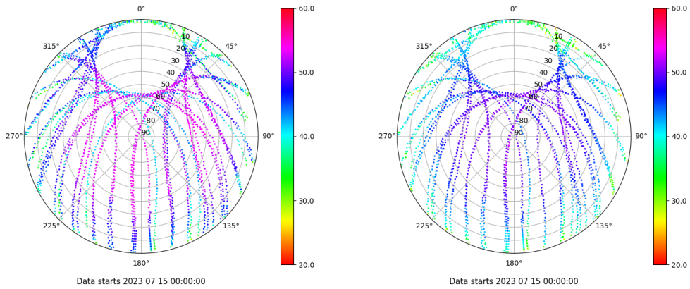
Skyplot for station SALA. Signal to Noise S1C Data file SALA00ESP_R_2023196.xtr Skyplot for station SALA. Signal to Noise S2P Data file SALA00ESP_R_2023196.xtr
