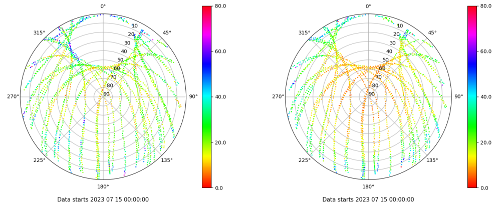
Skyplot for station SALA. Parameter M1C Data file SALA00ESP_R_2023196.xtr Skyplot for station SALA. Parameter M2P Data file SALA00ESP_R_2023196.xtr
