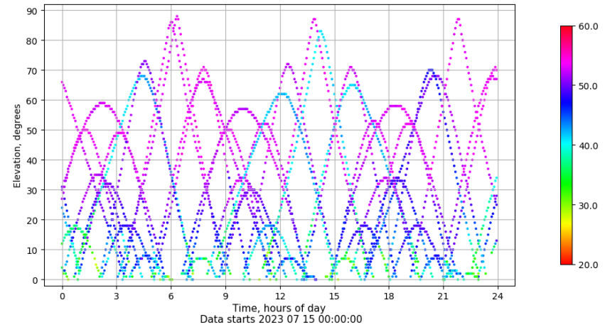
Time-elevation plot for station SALA. Signal to Noise S1C Data file SALA00ESP_R_2023196.xtr
