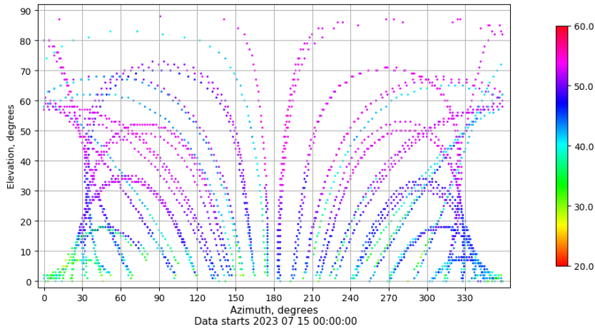
Azimuth-elevation plot for station SALA. Signal to Noise S1C Data file SALA00ESP_R_2023196.xtr
