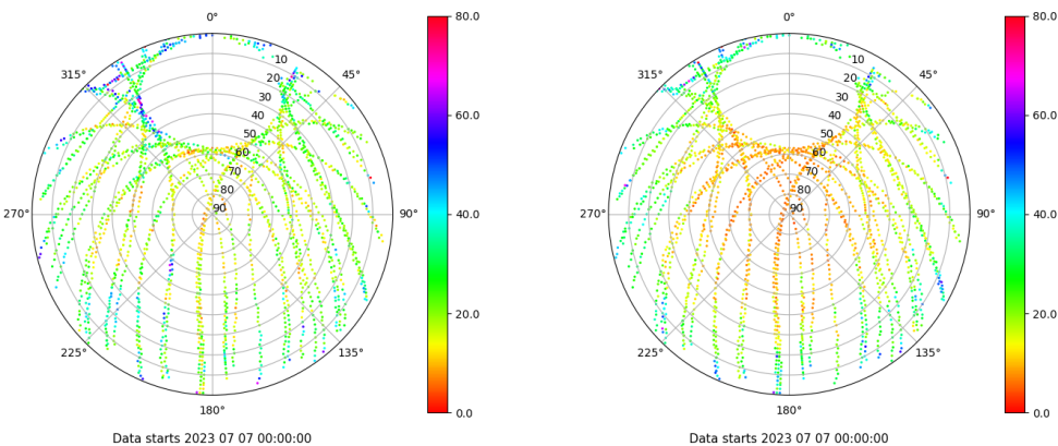
Skyplot for station SALA. Parameter M1C Data file SALA00ESP_R_2023188.xtr Skyplot for station SALA. Parameter M2P Data file SALA00ESP_R_2023188.xtr
