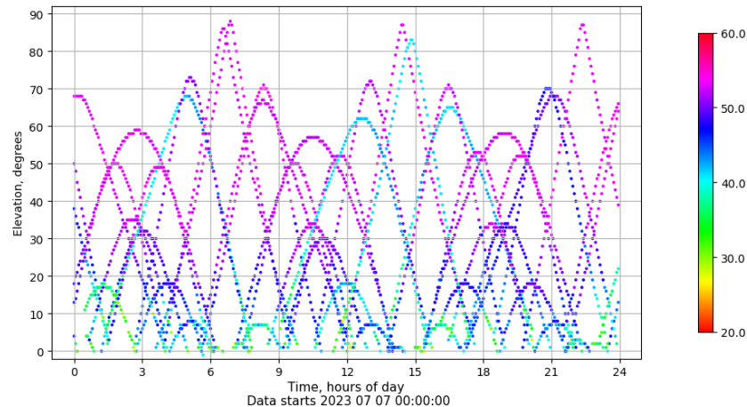
Time-elevation plot for station SALA. Signal to Noise S1C Data file SALA00ESP_R_2023188.xtr
