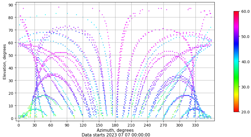
Azimuth-elevation plot for station SALA. Signal to Noise S1C Data file SALA00ESP_R_2023188.xtr
