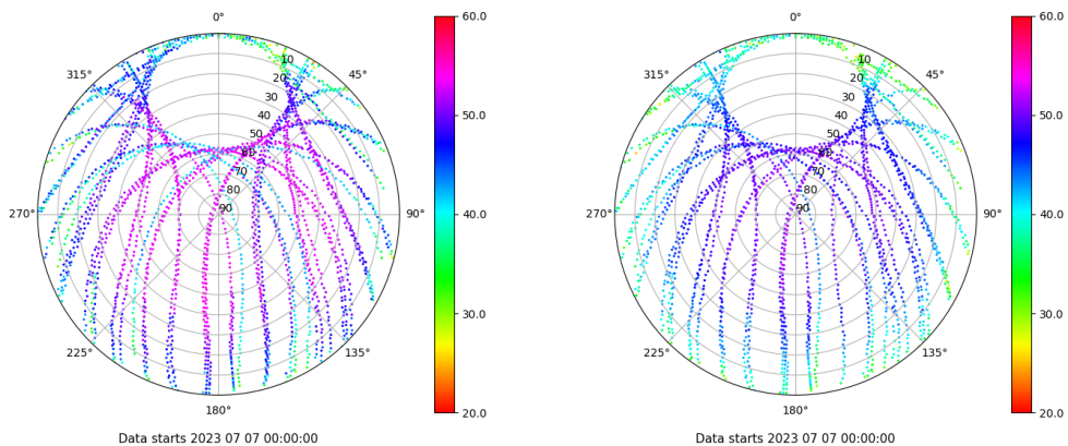
Skyplot for station SALA. Signal to Noise S1C Data file SALA00ESP_R_2023188.xtr Skyplot for station SALA. Signal to Noise S2P Data file SALA00ESP_R_2023188.xtr
