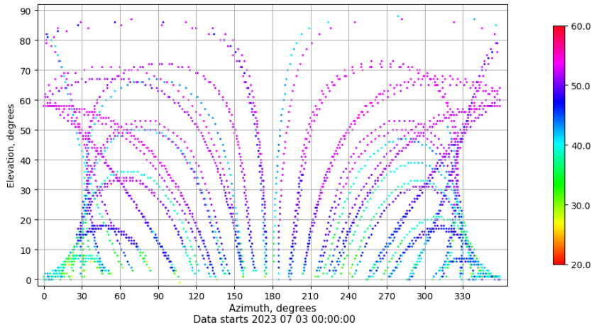
Azimuth-elevation plot for station SALA. Signal to Noise S1C Data file SALA00ESP_R_2023184.xtr
