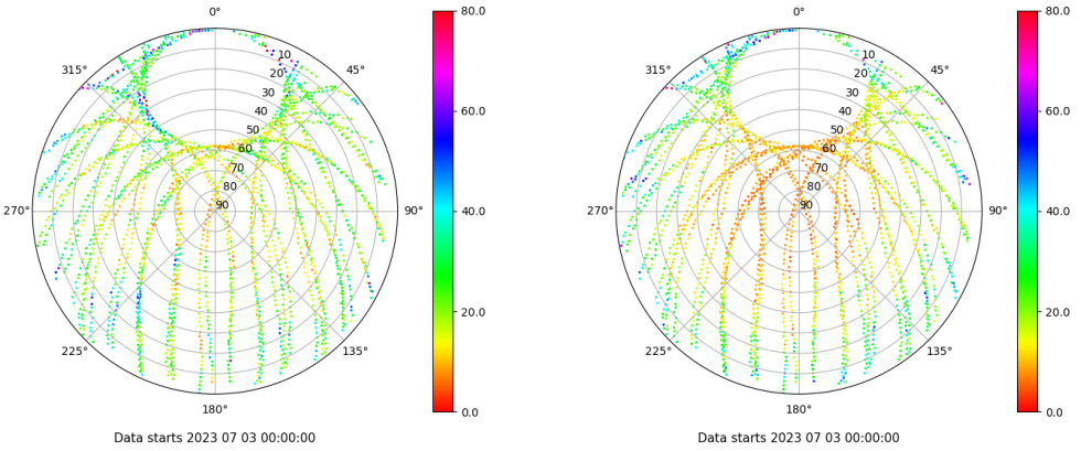
Skyplot for station SALA. Parameter M1C Data file SALA00ESP_R_2023184.xtr Skyplot for station SALA. Parameter M2P Data file SALA00ESP_R_2023184.xtr
