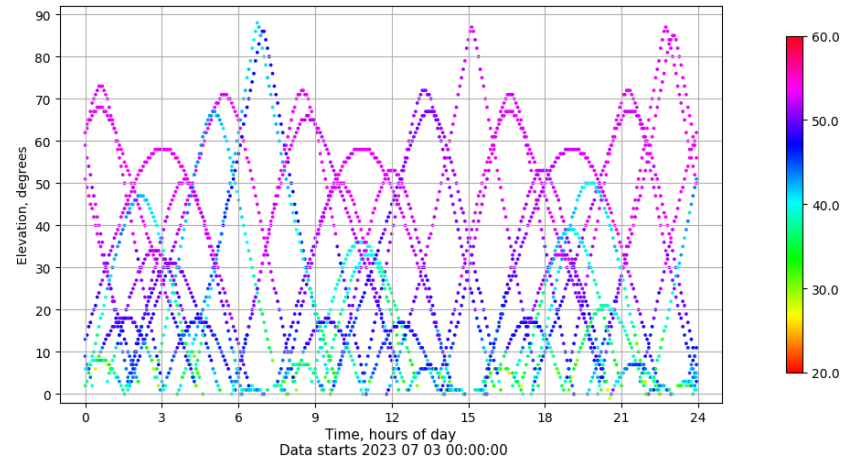
Time-elevation plot for station SALA. Signal to Noise S1C Data file SALA00ESP_R_2023184.xtr
