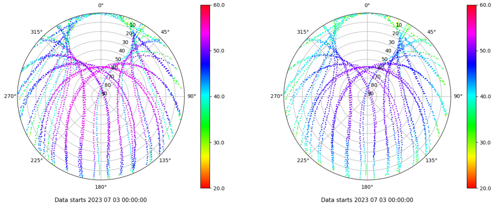
Skyplot for station SALA. Signal to Noise S1C Data file SALA00ESP_R_2023184.xtr Skyplot for station SALA. Signal to Noise S2P Data file SALA00ESP_R_2023184.xtr
