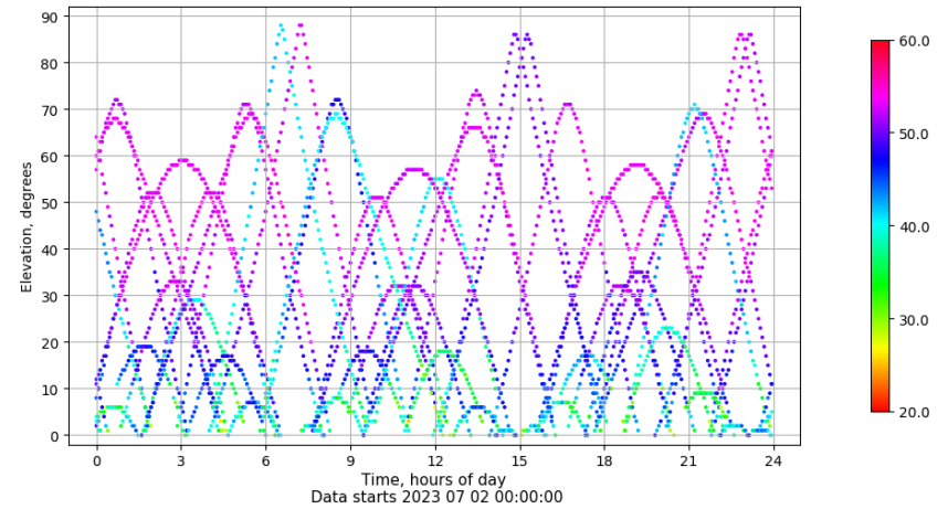
Time-elevation plot for station SALA. Signal to Noise S1C Data file SALA00ESP_R_2023183.xtr
