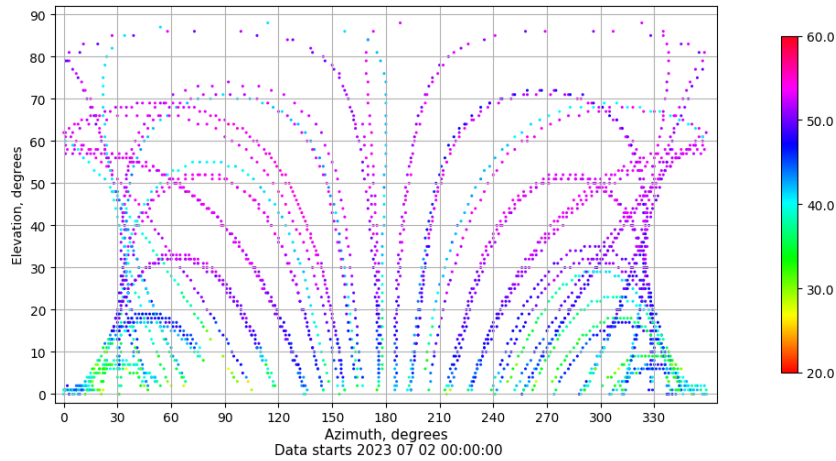
Azimuth-elevation plot for station SALA. Signal to Noise S1C Data file SALA00ESP_R_2023183.xtr
