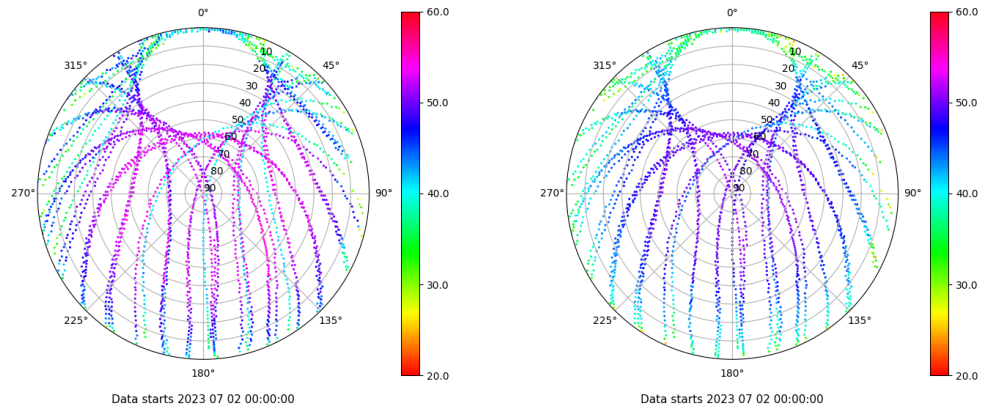
Skyplot for station SALA. Signal to Noise S1C Data file SALA00ESP_R_2023183.xtr Skyplot for station SALA. Signal to Noise S2P Data file SALA00ESP_R_2023183.xtr
