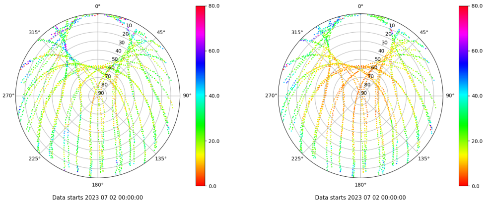
Skyplot for station SALA. Parameter M1C Data file SALA00ESP_R_2023183.xtr Skyplot for station SALA. Parameter M2P Data file SALA00ESP_R_2023183.xtr
