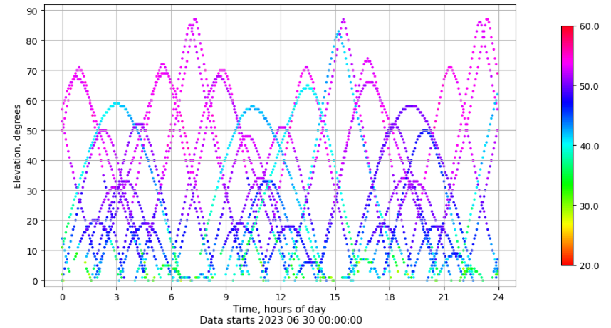
Time-elevation plot for station SALA. Signal to Noise S1C Data file SALA00ESP_R_2023181.xtr
