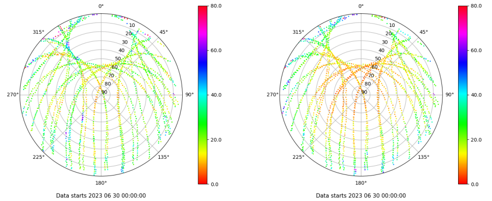
Skyplot for station SALA. Parameter M1C Data file SALA00ESP_R_2023181.xtr Skyplot for station SALA. Parameter M2P Data file SALA00ESP_R_2023181.xtr
