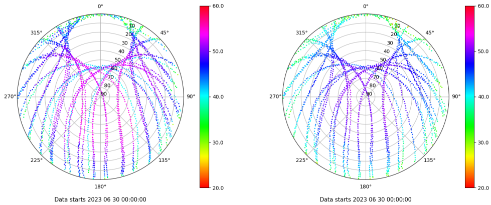
Skyplot for station SALA. Signal to Noise S1C Data file SALA00ESP_R_2023181.xtr Skyplot for station SALA. Signal to Noise S2P Data file SALA00ESP_R_2023181.xtr
