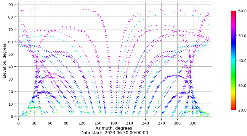
Azimuth-elevation plot for station SALA. Signal to Noise S1C Data file SALA00ESP_R_2023181.xtr
