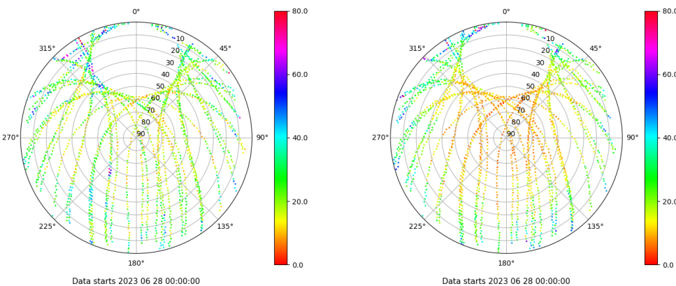
Skyplot for station SALA. Parameter M1C Data file SALA00ESP_R_2023179.xtr Skyplot for station SALA. Parameter M2P Data file SALA00ESP_R_2023179.xtr
