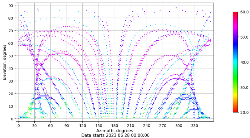
Azimuth-elevation plot for station SALA. Signal to Noise S1C Data file SALA00ESP_R_2023179.xtr
