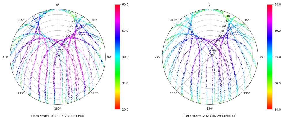
Skyplot for station SALA. Signal to Noise S1C Data file SALA00ESP_R_2023179.xtr Skyplot for station SALA. Signal to Noise S2P Data file SALA00ESP_R_2023179.xtr
