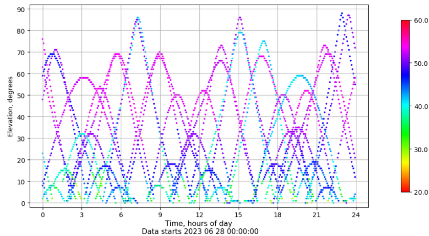
Time-elevation plot for station SALA. Signal to Noise S1C Data file SALA00ESP_R_2023179.xtr
