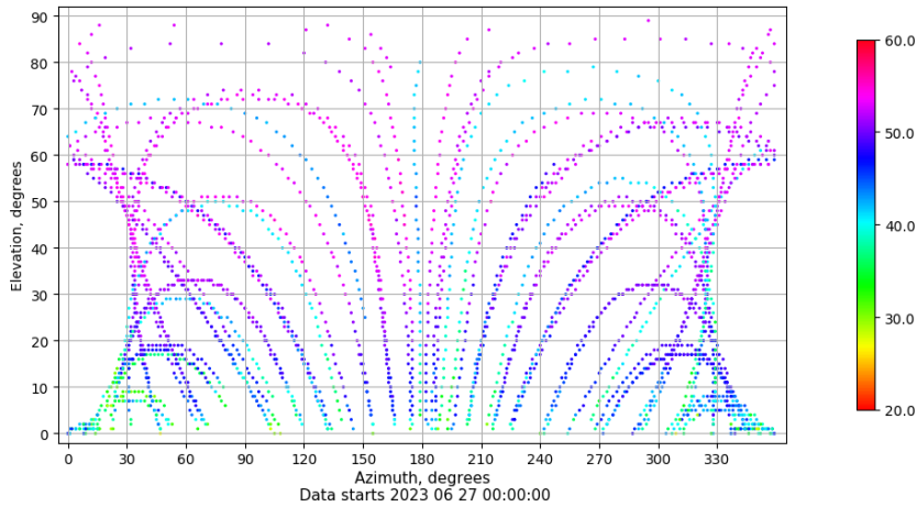
Azimuth-elevation plot for station SALA. Signal to Noise S1C Data file SALA00ESP_R_2023178.xtr
