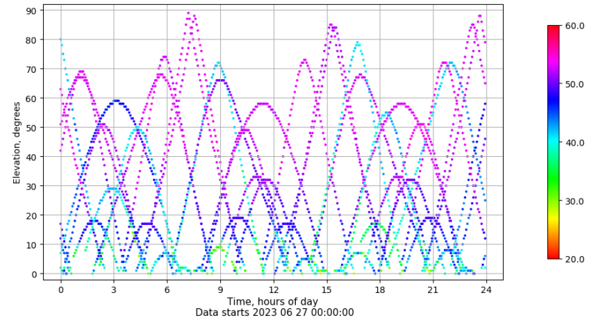
Time-elevation plot for station SALA. Signal to Noise S1C Data file SALA00ESP_R_2023178.xtr
