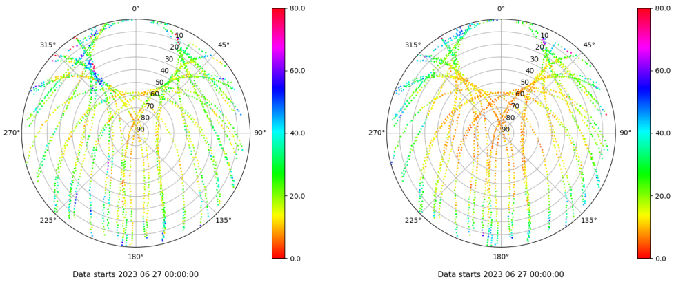
Skyplot for station SALA. Parameter M1C Data file SALA00ESP_R_2023178.xtr Skyplot for station SALA. Parameter M2P Data file SALA00ESP_R_2023178.xtr
