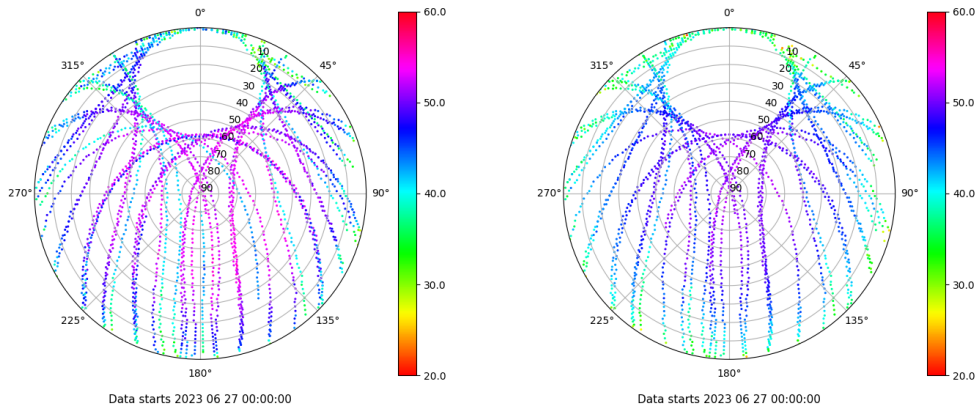
Skyplot for station SALA. Signal to Noise S1C Data file SALA00ESP_R_2023178.xtr Skyplot for station SALA. Signal to Noise S2P Data file SALA00ESP_R_2023178.xtr
