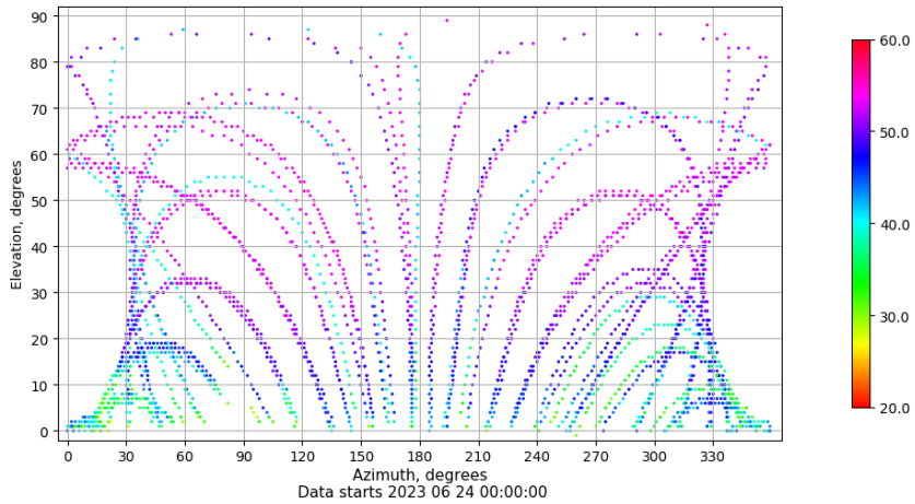
Azimuth-elevation plot for station SALA. Signal to Noise S1C Data file SALA00ESP_R_2023175.xtr
