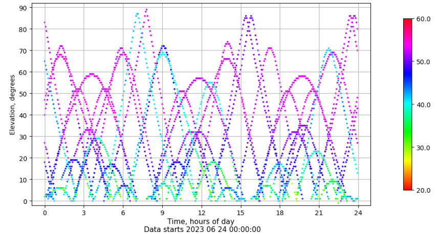
Time-elevation plot for station SALA. Signal to Noise S1C Data file SALA00ESP_R_2023175.xtr
