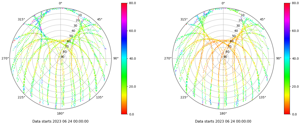
Skyplot for station SALA. Parameter M1C Data file SALA00ESP_R_2023175.xtr Skyplot for station SALA. Parameter M2P Data file SALA00ESP_R_2023175.xtr
