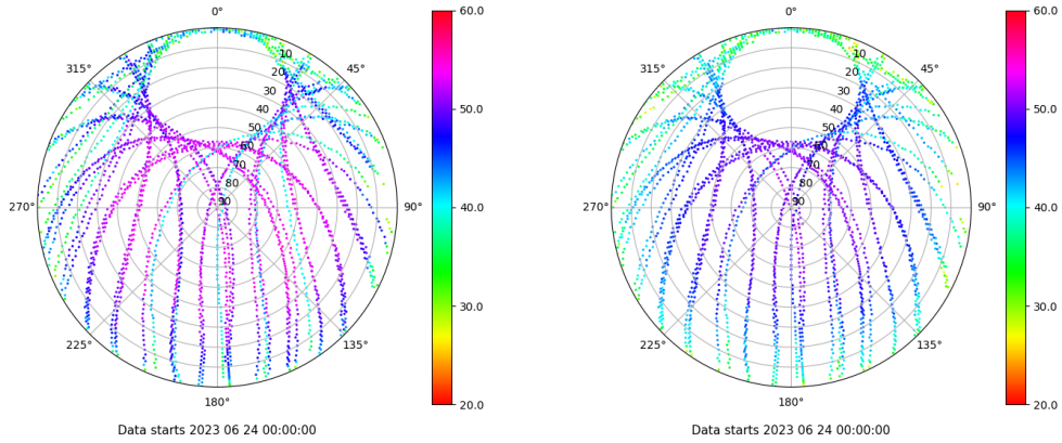
Skyplot for station SALA. Signal to Noise S1C Data file SALA00ESP_R_2023175.xtr Skyplot for station SALA. Signal to Noise S2P Data file SALA00ESP_R_2023175.xtr
