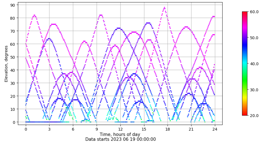
Time-elevation plot for station SALA. Signal to Noise S1C Data file SALA00ESP_R_2023170.xtr
