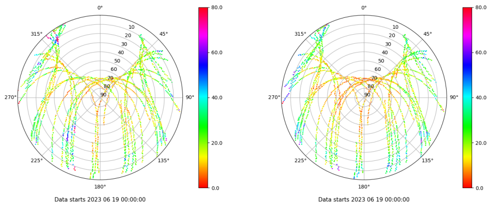
Skyplot for station SALA. Parameter M1C Data file SALA00ESP_R_2023170.xtr Skyplot for station SALA. Parameter M5Q Data file SALA00ESP_R_2023170.xtr
