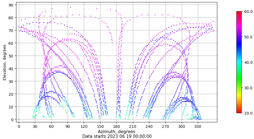
Azimuth-elevation plot for station SALA. Signal to Noise S1C Data file SALA00ESP_R_2023170.xtr
