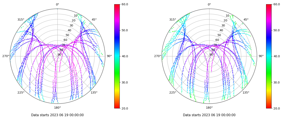
Skyplot for station SALA. Signal to Noise S1C Data file SALA00ESP_R_2023170.xtr Skyplot for station SALA. Signal to Noise S5Q Data file SALA00ESP_R_2023170.xtr
