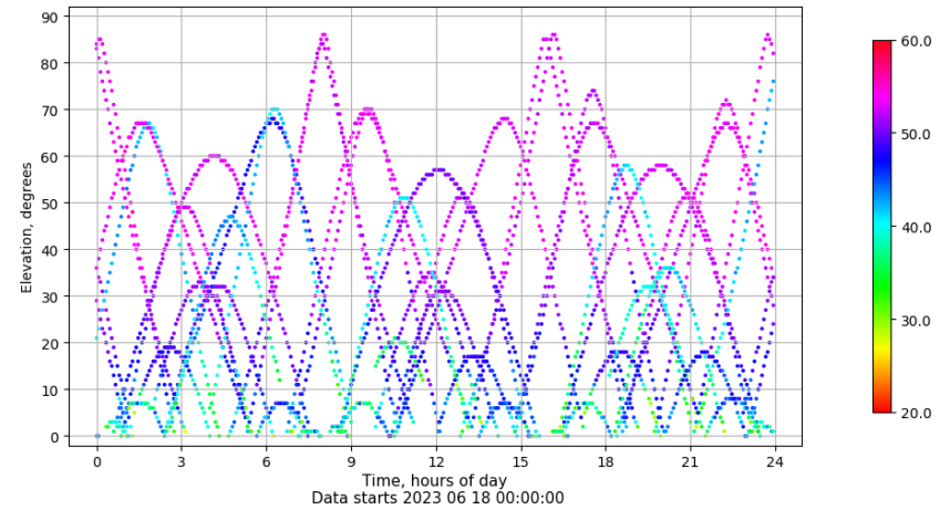
Time-elevation plot for station SALA. Signal to Noise S1C Data file SALA00ESP_R_2023169.xtr
