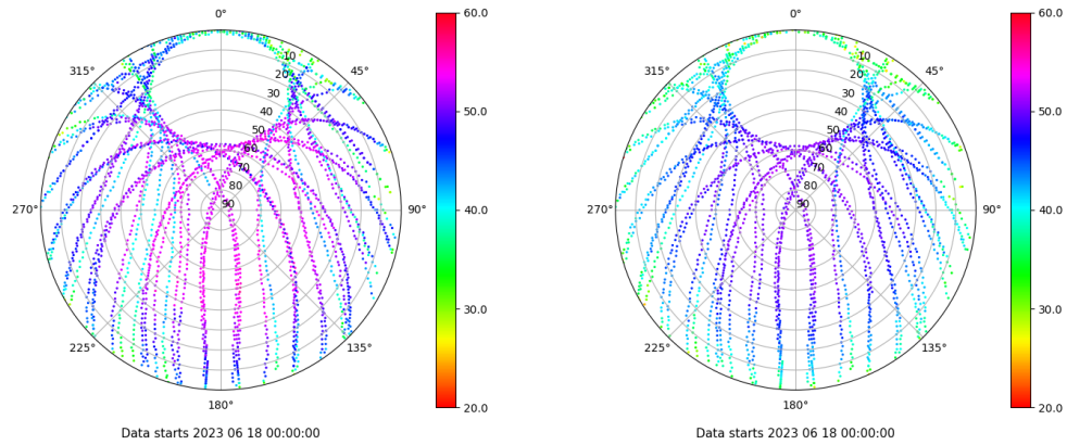
Skyplot for station SALA. Signal to Noise S1C Data file SALA00ESP_R_2023169.xtr Skyplot for station SALA. Signal to Noise S2P Data file SALA00ESP_R_2023169.xtr
