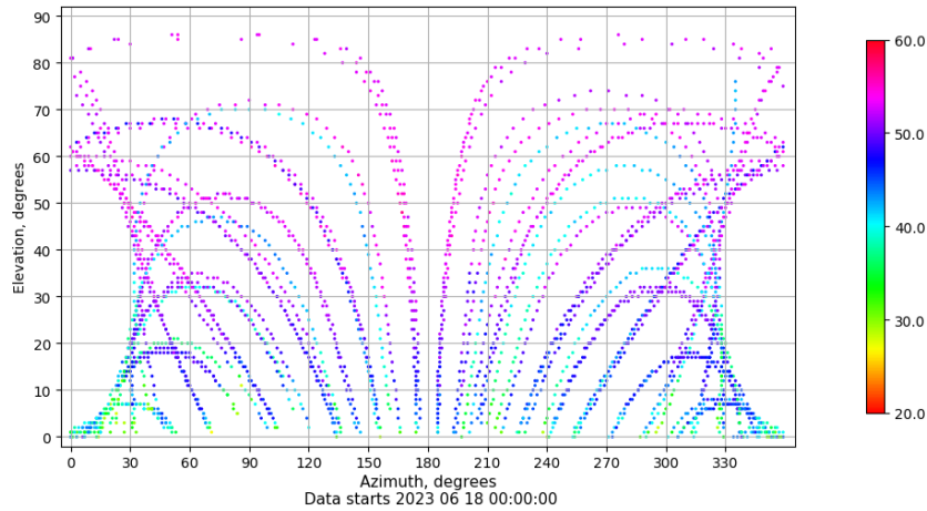
Azimuth-elevation plot for station SALA. Signal to Noise S1C Data file SALA00ESP_R_2023169.xtr
