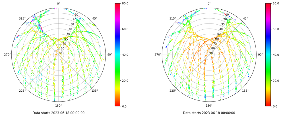
Skyplot for station SALA. Parameter M1C Data file SALA00ESP_R_2023169.xtr Skyplot for station SALA. Parameter M2P Data file SALA00ESP_R_2023169.xtr
