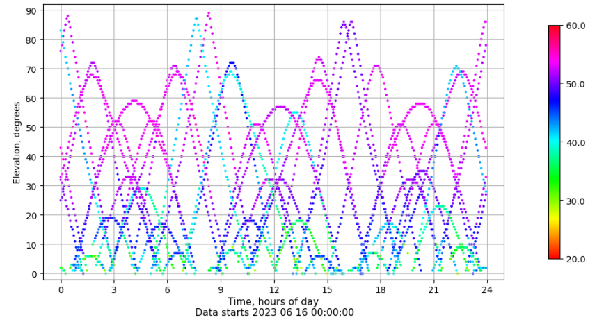
Time-elevation plot for station SALA. Signal to Noise S1C Data file SALA00ESP_R_2023167.xtr
