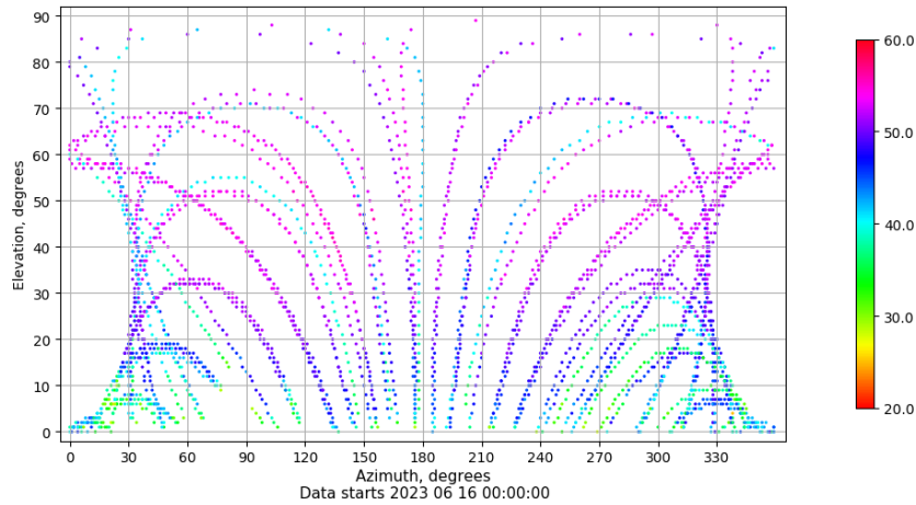
Azimuth-elevation plot for station SALA. Signal to Noise S1C Data file SALA00ESP_R_2023167.xtr
