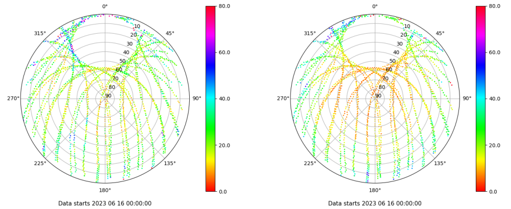
Skyplot for station SALA. Parameter M1C Data file SALA00ESP_R_2023167.xtr Skyplot for station SALA. Parameter M2P Data file SALA00ESP_R_2023167.xtr
