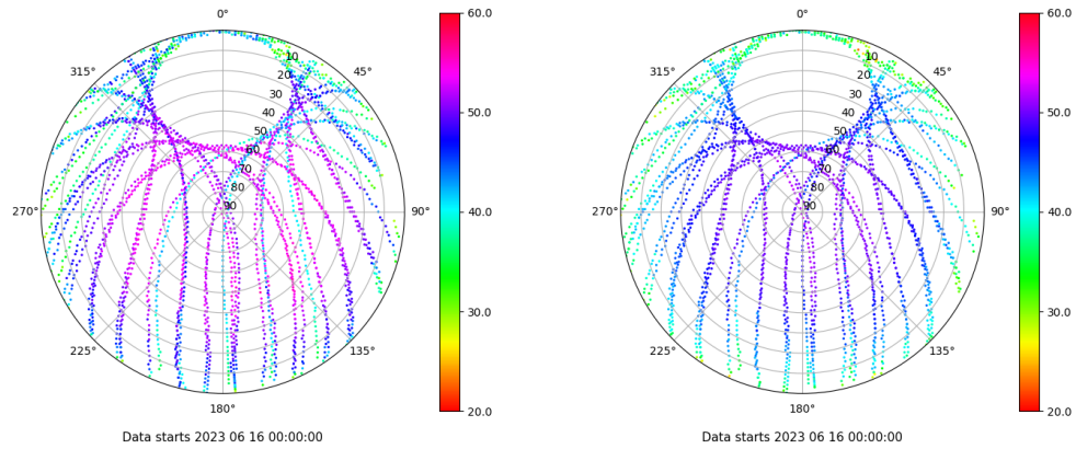
Skyplot for station SALA. Signal to Noise S1C Data file SALA00ESP_R_2023167.xtr Skyplot for station SALA. Signal to Noise S2P Data file SALA00ESP_R_2023167.xtr
