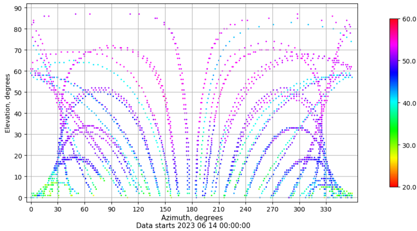
Azimuth-elevation plot for station SALA. Signal to Noise S1C Data file SALA00ESP_R_2023165.xtr
