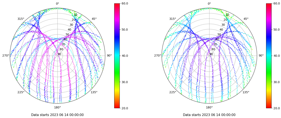
Skyplot for station SALA. Signal to Noise S1C Data file SALA00ESP_R_2023165.xtr Skyplot for station SALA. Signal to Noise S2P Data file SALA00ESP_R_2023165.xtr
