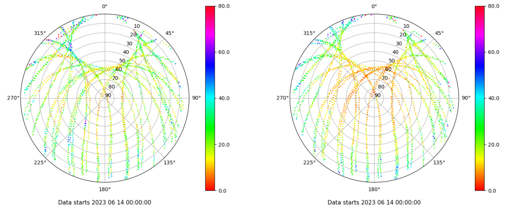
Skyplot for station SALA. Parameter M1C Data file SALA00ESP_R_2023165.xtr Skyplot for station SALA. Parameter M2P Data file SALA00ESP_R_2023165.xtr
