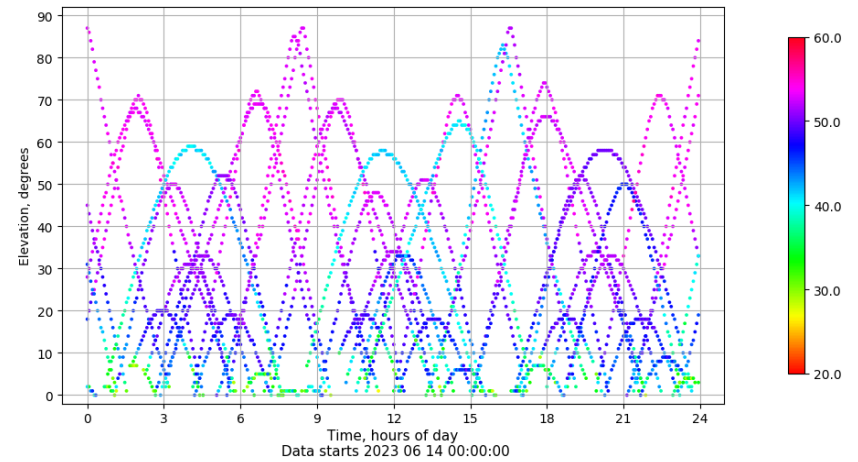
Time-elevation plot for station SALA. Signal to Noise S1C Data file SALA00ESP_R_2023165.xtr
