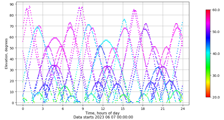
Time-elevation plot for station SALA. Signal to Noise S1C Data file SALA00ESP_R_2023158.xtr
