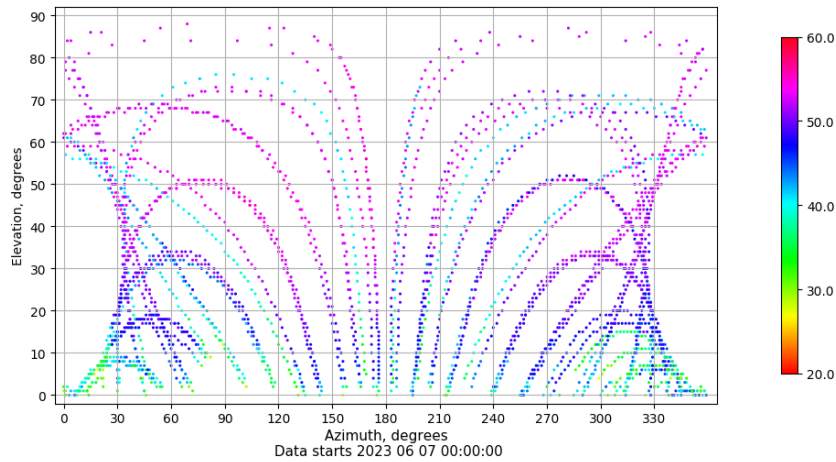
Azimuth-elevation plot for station SALA. Signal to Noise S1C Data file SALA00ESP_R_2023158.xtr
