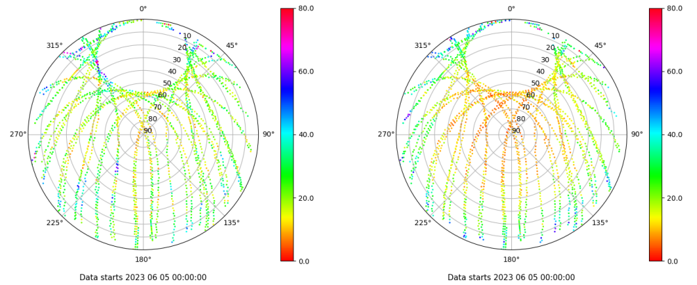
Skyplot for station SALA. Parameter M1C Data file SALA00ESP_R_2023156.xtr Skyplot for station SALA. Parameter M2P Data file SALA00ESP_R_2023156.xtr
