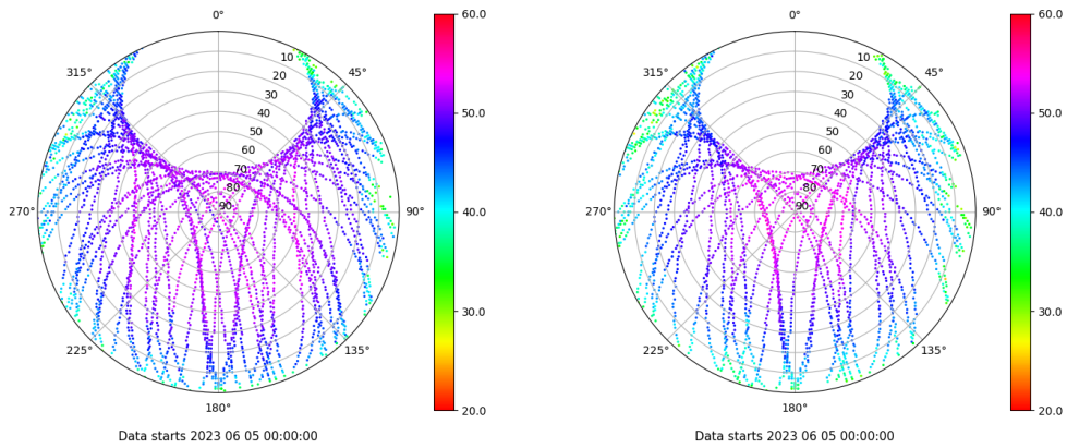
Skyplot for station SALA. Signal to Noise S1C Data file SALA00ESP_R_2023156.xtr Skyplot for station SALA. Signal to Noise S2S Data file SALA00ESP_R_2023156.xtr
