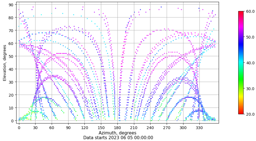
Azimuth-elevation plot for station SALA. Signal to Noise S1C Data file SALA00ESP_R_2023156.xtr
