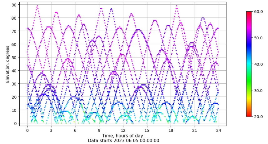
Time-elevation plot for station SALA. Signal to Noise S1C Data file SALA00ESP_R_2023156.xtr
