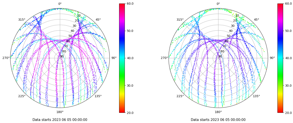
Skyplot for station SALA. Signal to Noise S1C Data file SALA00ESP_R_2023156.xtr Skyplot for station SALA. Signal to Noise S2P Data file SALA00ESP_R_2023156.xtr
