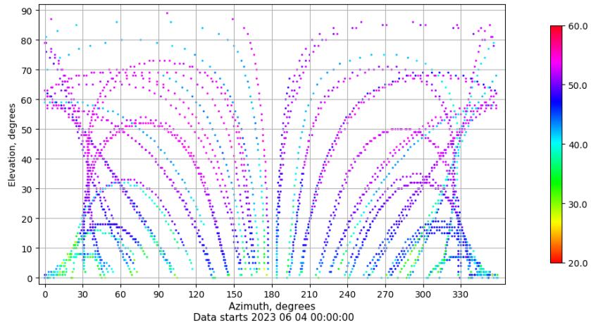
Azimuth-elevation plot for station SALA. Signal to Noise S1C Data file SALA00ESP_R_2023155.xtr
