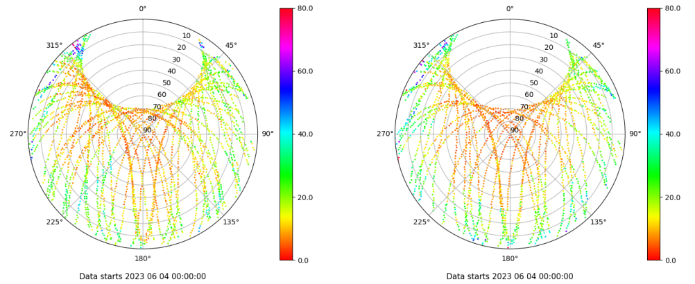
Skyplot for station SALA. Parameter M1C Data file SALA00ESP_R_2023155.xtr Skyplot for station SALA. Parameter M2S Data file SALA00ESP_R_2023155.xtr
