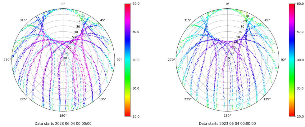
Skyplot for station SALA. Signal to Noise S1C Data file SALA00ESP_R_2023155.xtr Skyplot for station SALA. Signal to Noise S2P Data file SALA00ESP_R_2023155.xtr
