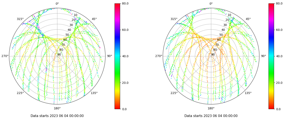
Skyplot for station SALA. Parameter M1C Data file SALA00ESP_R_2023155.xtr Skyplot for station SALA. Parameter M2P Data file SALA00ESP_R_2023155.xtr
