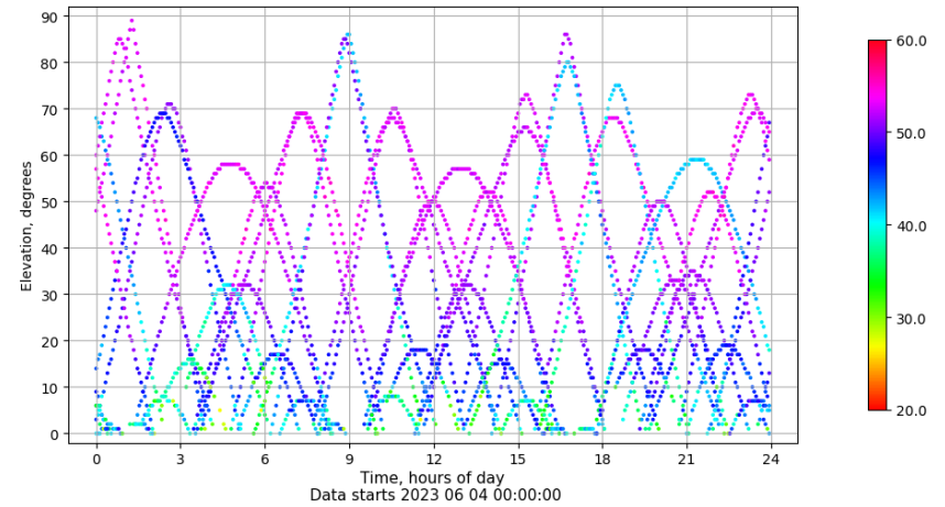
Time-elevation plot for station SALA. Signal to Noise S1C Data file SALA00ESP_R_2023155.xtr
