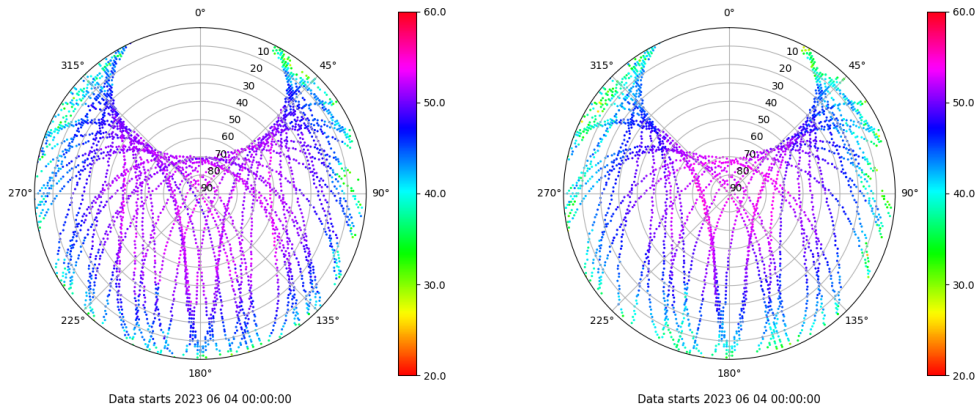
Skyplot for station SALA. Signal to Noise S1C Data file SALA00ESP_R_2023155.xtr Skyplot for station SALA. Signal to Noise S2S Data file SALA00ESP_R_2023155.xtr
