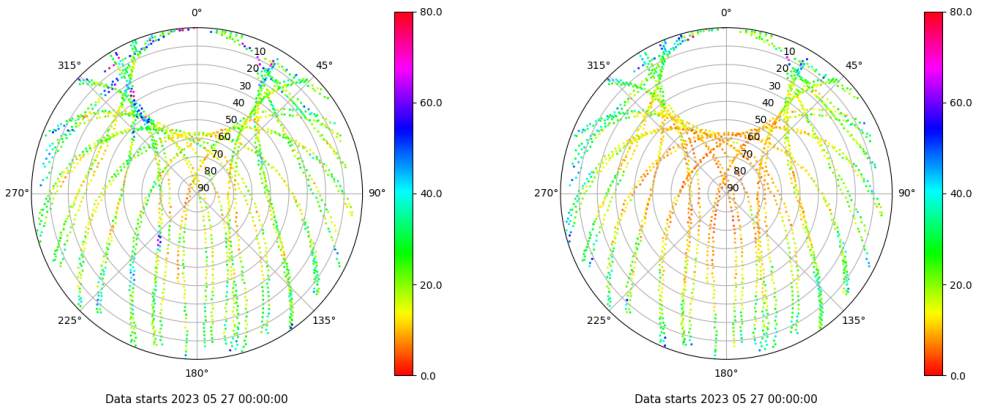
Skyplot for station SALA. Parameter M1C Data file SALA00ESP_R_2023147.xtr Skyplot for station SALA. Parameter M2P Data file SALA00ESP_R_2023147.xtr
