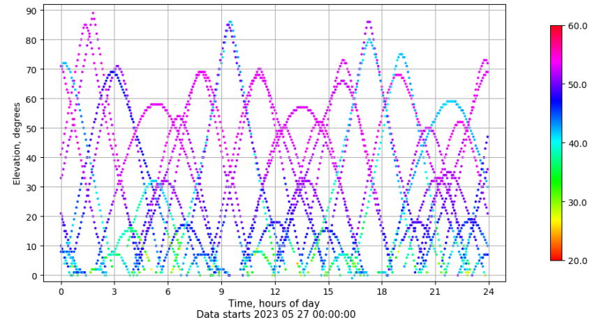
Time-elevation plot for station SALA. Signal to Noise S1C Data file SALA00ESP_R_2023147.xtr
