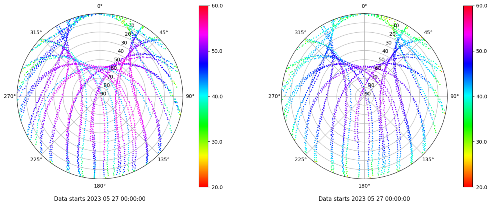
Skyplot for station SALA. Signal to Noise S1C Data file SALA00ESP_R_2023147.xtr Skyplot for station SALA. Signal to Noise S2P Data file SALA00ESP_R_2023147.xtr
