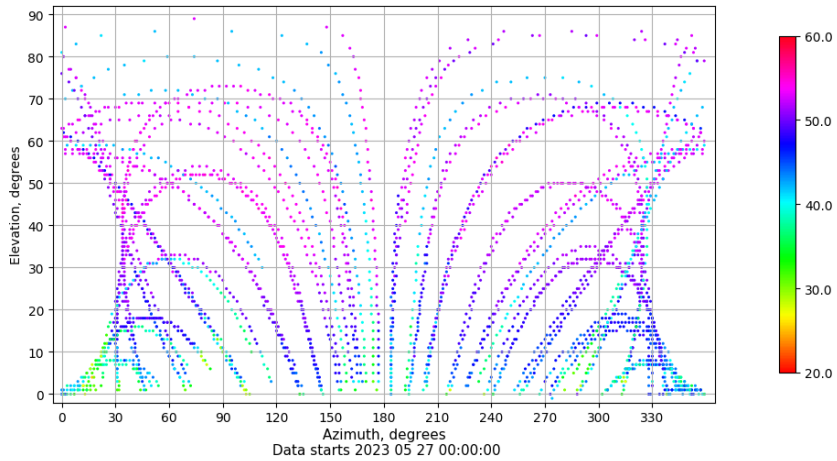
Azimuth-elevation plot for station SALA. Signal to Noise S1C Data file SALA00ESP_R_2023147.xtr
