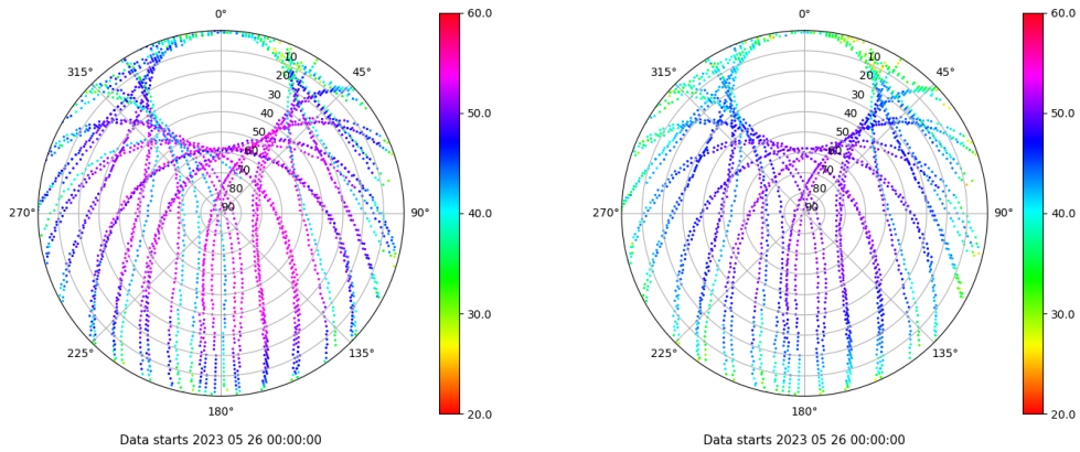
Skyplot for station SALA. Signal to Noise S1C Data file SALA00ESP_R_2023146.xtr Skyplot for station SALA. Signal to Noise S2P Data file SALA00ESP_R_2023146.xtr
