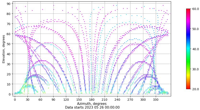
Azimuth-elevation plot for station SALA. Signal to Noise S1C Data file SALA00ESP_R_2023146.xtr
