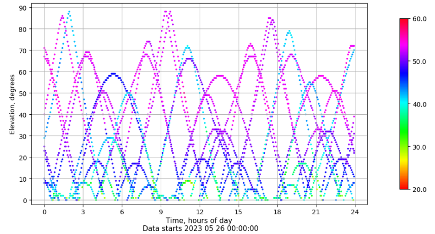
Time-elevation plot for station SALA. Signal to Noise S1C Data file SALA00ESP_R_2023146.xtr
