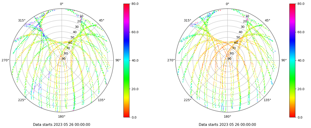
Skyplot for station SALA. Parameter M1C Data file SALA00ESP_R_2023146.xtr Skyplot for station SALA. Parameter M2P Data file SALA00ESP_R_2023146.xtr
