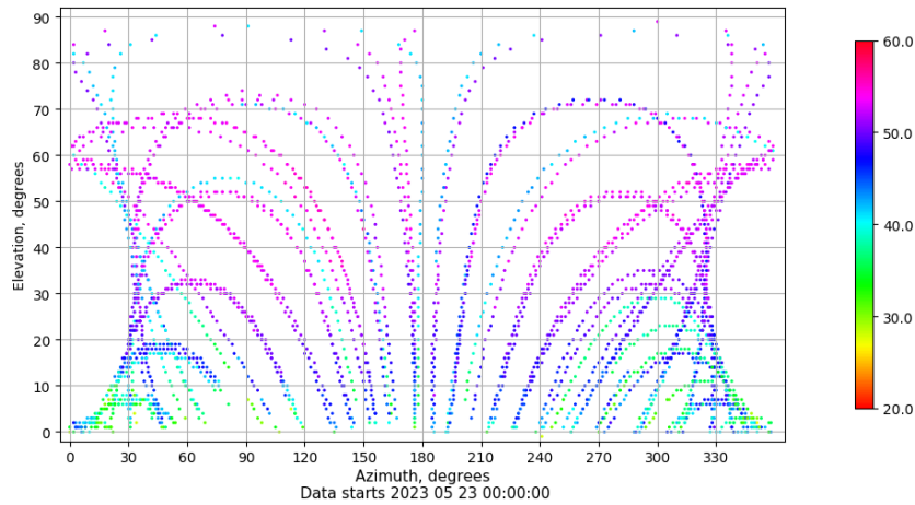
Azimuth-elevation plot for station SALA. Signal to Noise S1C Data file SALA00ESP_R_2023143.xtr
