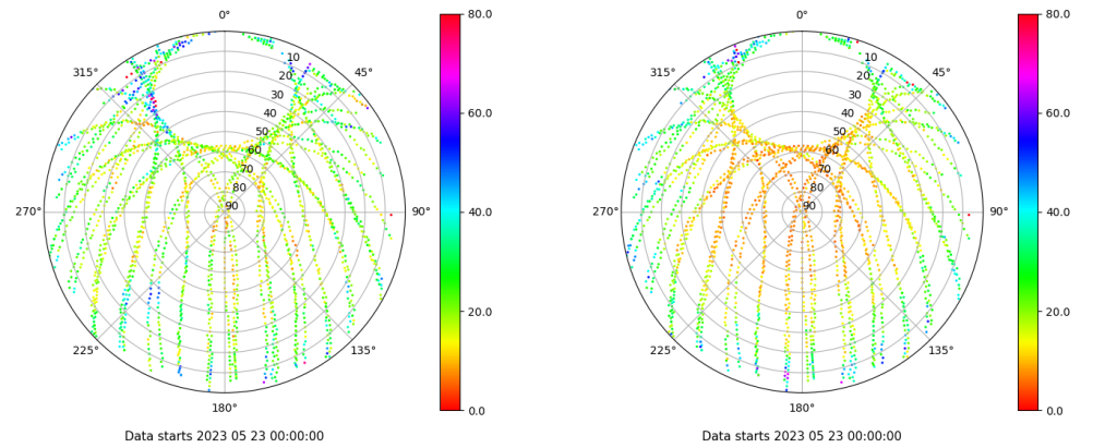
Skyplot for station SALA. Parameter M1C Data file SALA00ESP_R_2023143.xtr Skyplot for station SALA. Parameter M2P Data file SALA00ESP_R_2023143.xtr
