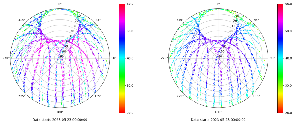
Skyplot for station SALA. Signal to Noise S1C Data file SALA00ESP_R_2023143.xtr Skyplot for station SALA. Signal to Noise S2P Data file SALA00ESP_R_2023143.xtr
