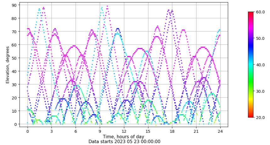
Time-elevation plot for station SALA. Signal to Noise S1C Data file SALA00ESP_R_2023143.xtr
