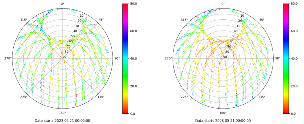
Skyplot for station SALA. Parameter M1C Data file SALA00ESP_R_2023141.xtr Skyplot for station SALA. Parameter M2P Data file SALA00ESP_R_2023141.xtr
