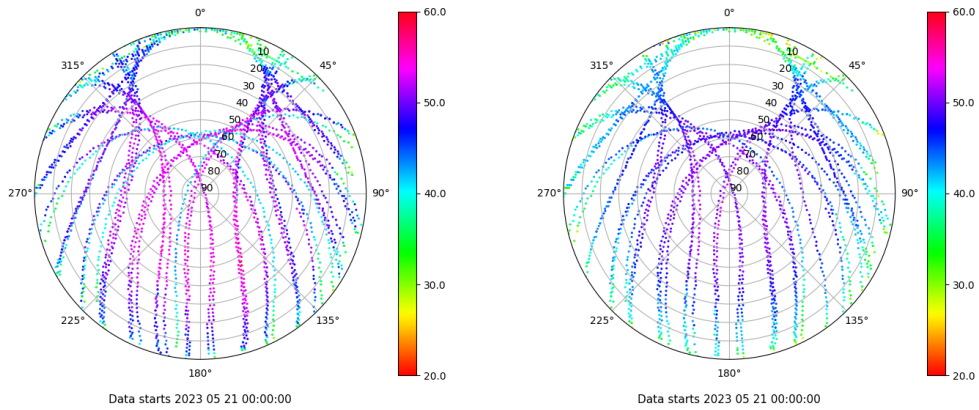
Skyplot for station SALA. Signal to Noise S1C Data file SALA00ESP_R_2023141.xtr Skyplot for station SALA. Signal to Noise S2P Data file SALA00ESP_R_2023141.xtr
