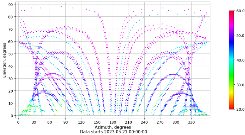
Azimuth-elevation plot for station SALA. Signal to Noise S1C Data file SALA00ESP_R_2023141.xtr
