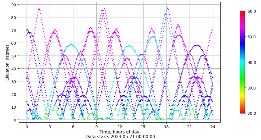
Time-elevation plot for station SALA. Signal to Noise S1C Data file SALA00ESP_R_2023141.xtr
