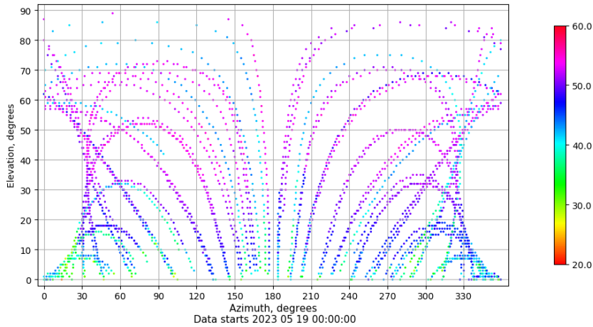
Azimuth-elevation plot for station SALA. Signal to Noise S1C Data file SALA00ESP_R_2023139.xtr
