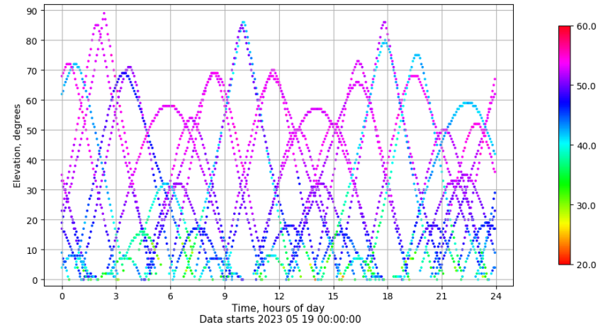
Time-elevation plot for station SALA. Signal to Noise S1C Data file SALA00ESP_R_2023139.xtr
