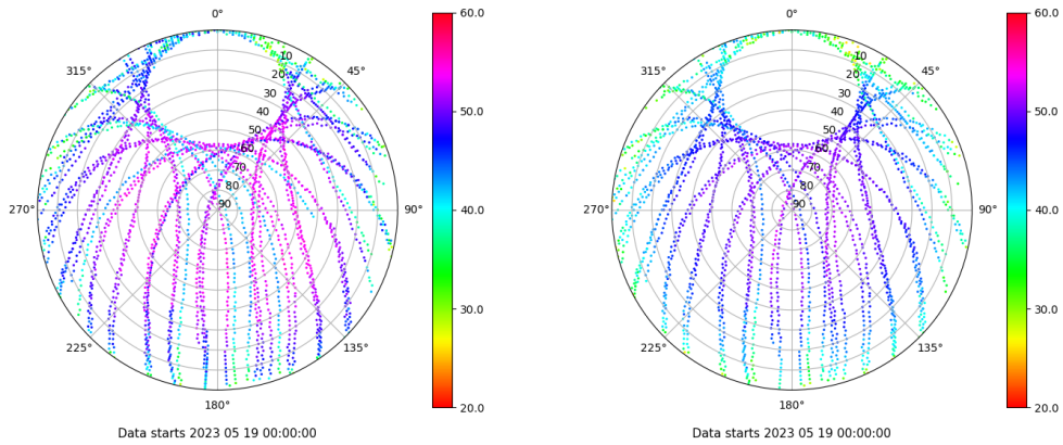
Skyplot for station SALA. Signal to Noise S1C Data file SALA00ESP_R_2023139.xtr Skyplot for station SALA. Signal to Noise S2P Data file SALA00ESP_R_2023139.xtr
