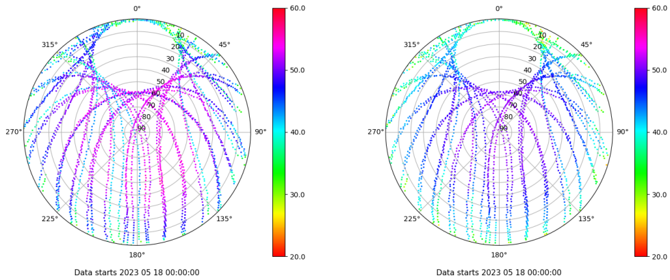
Skyplot for station SALA. Signal to Noise S1C Data file SALA00ESP_R_2023138.xtr Skyplot for station SALA. Signal to Noise S2P Data file SALA00ESP_R_2023138.xtr
