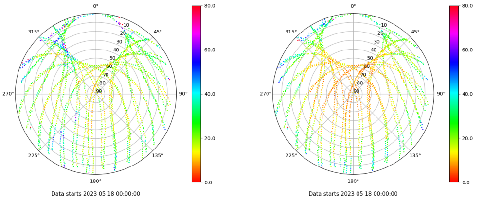
Skyplot for station SALA. Parameter M1C Data file SALA00ESP_R_2023138.xtr Skyplot for station SALA. Parameter M2P Data file SALA00ESP_R_2023138.xtr
