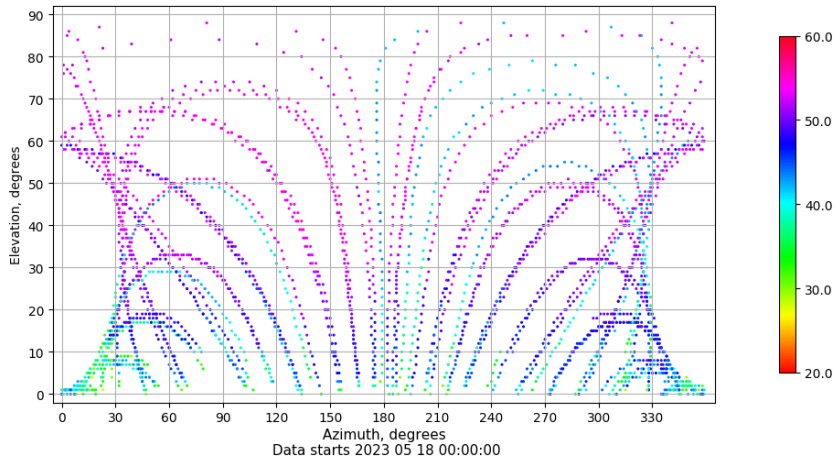
Azimuth-elevation plot for station SALA. Signal to Noise S1C Data file SALA00ESP_R_2023138.xtr
