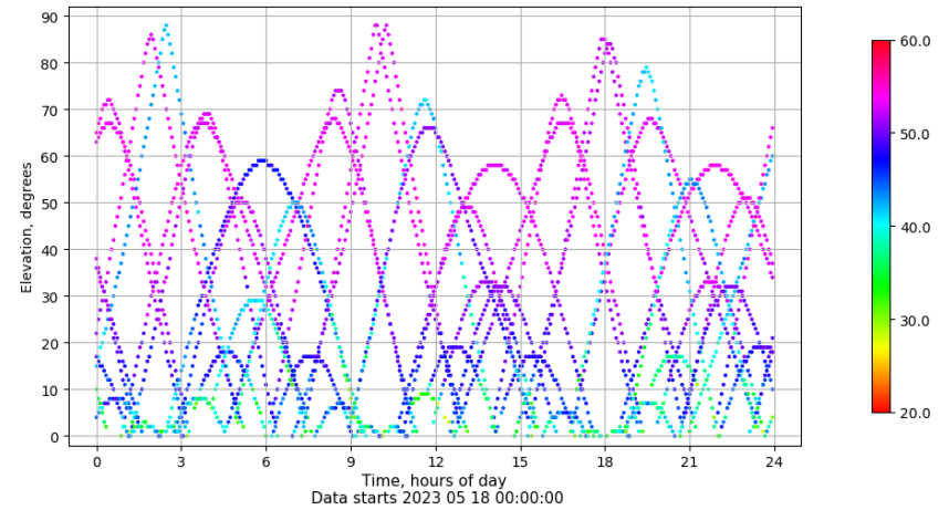
Time-elevation plot for station SALA. Signal to Noise S1C Data file SALA00ESP_R_2023138.xtr
