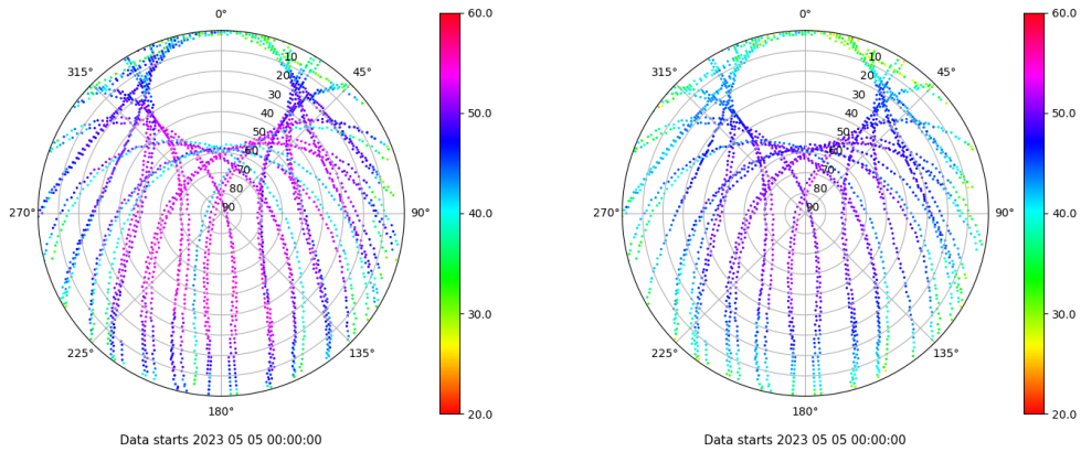
Skyplot for station SALA. Signal to Noise S1C Data file SALA00ESP_R_2023125.xtr Skyplot for station SALA. Signal to Noise S2P Data file SALA00ESP_R_2023125.xtr
