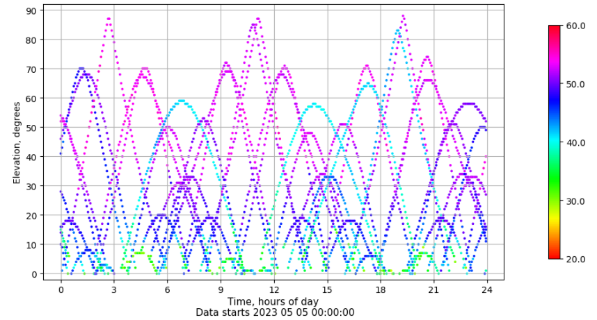
Time-elevation plot for station SALA. Signal to Noise S1C Data file SALA00ESP_R_2023125.xtr
