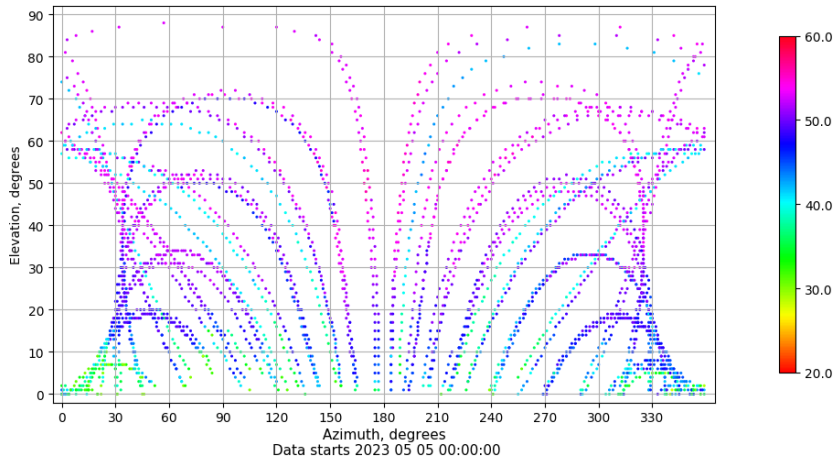
Azimuth-elevation plot for station SALA. Signal to Noise S1C Data file SALA00ESP_R_2023125.xtr
