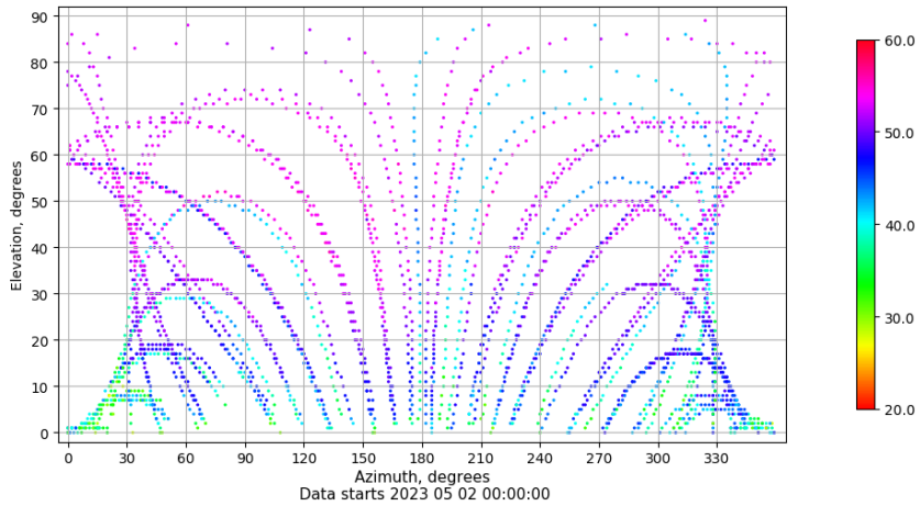
Azimuth-elevation plot for station SALA. Signal to Noise S1C Data file SALA00ESP_R_2023122.xtr
