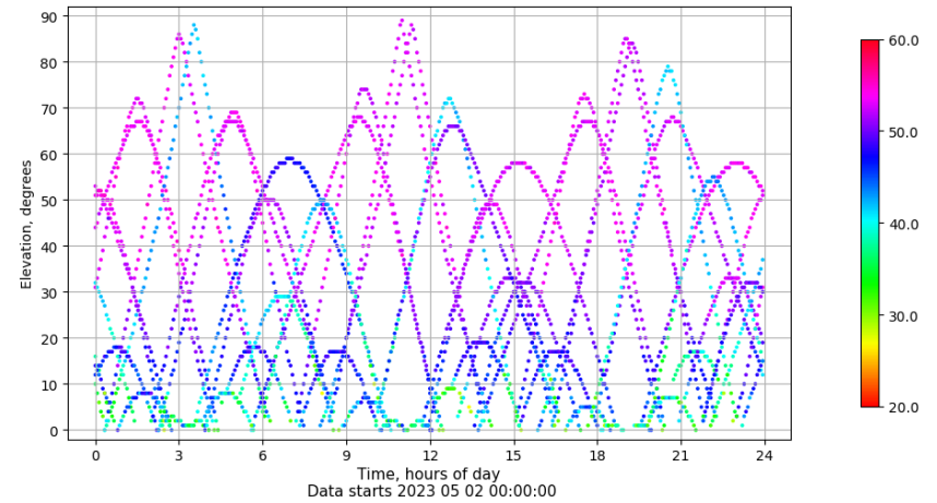
Time-elevation plot for station SALA. Signal to Noise S1C Data file SALA00ESP_R_2023122.xtr
