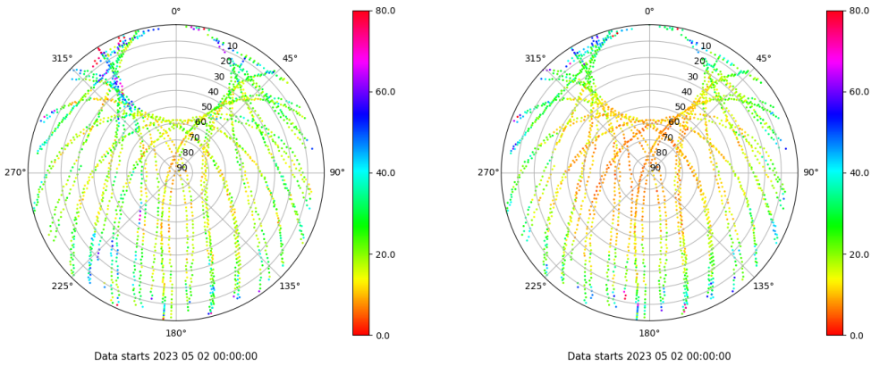
Skyplot for station SALA. Parameter M1C Data file SALA00ESP_R_2023122.xtr Skyplot for station SALA. Parameter M2P Data file SALA00ESP_R_2023122.xtr
