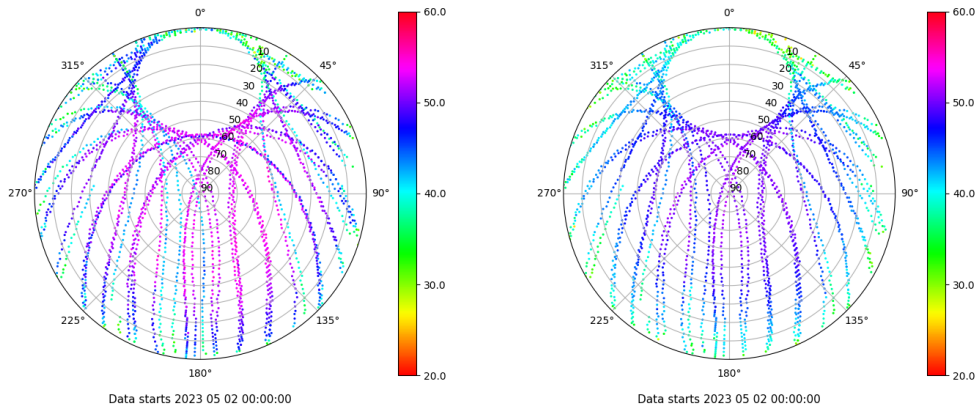
Skyplot for station SALA. Signal to Noise S1C Data file SALA00ESP_R_2023122.xtr Skyplot for station SALA. Signal to Noise S2P Data file SALA00ESP_R_2023122.xtr
