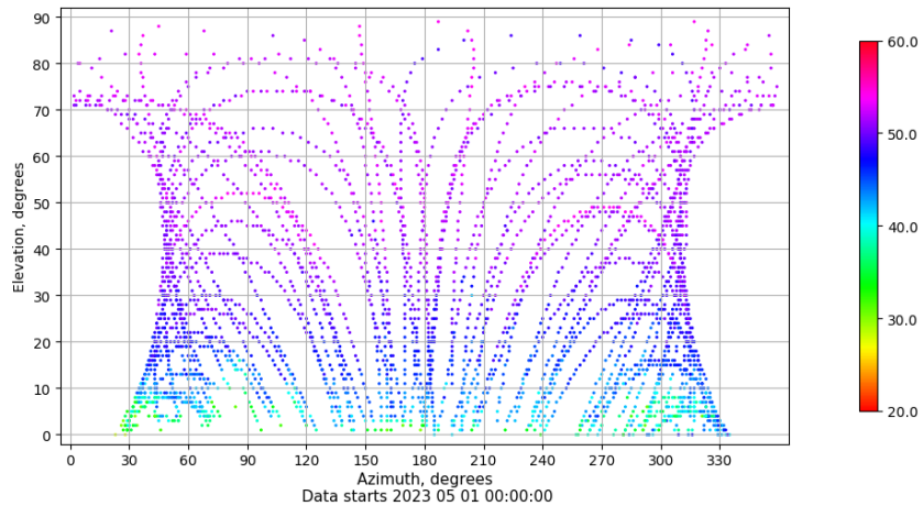
Azimuth-elevation plot for station SALA. Signal to Noise S1C Data file SALA00ESP_R_2023121.xtr
