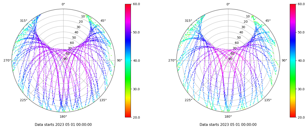
Skyplot for station SALA. Signal to Noise S1C Data file SALA00ESP_R_2023121.xtr Skyplot for station SALA. Signal to Noise S2S Data file SALA00ESP_R_2023121.xtr
