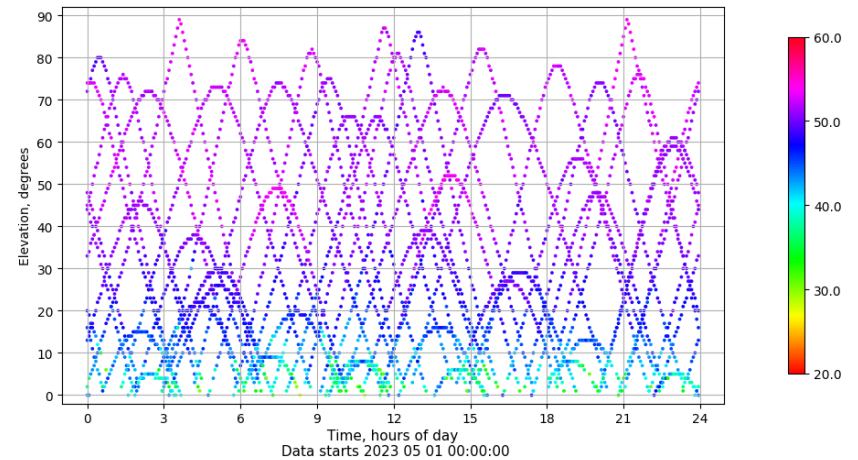
Time-elevation plot for station SALA. Signal to Noise S1C Data file SALA00ESP_R_2023121.xtr
