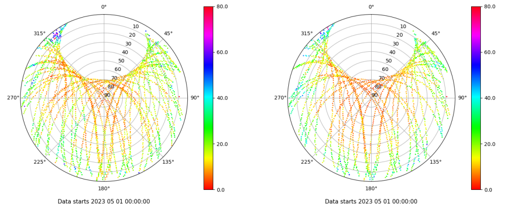
Skyplot for station SALA. Parameter M1C Data file SALA00ESP_R_2023121.xtr Skyplot for station SALA. Parameter M2S Data file SALA00ESP_R_2023121.xtr
