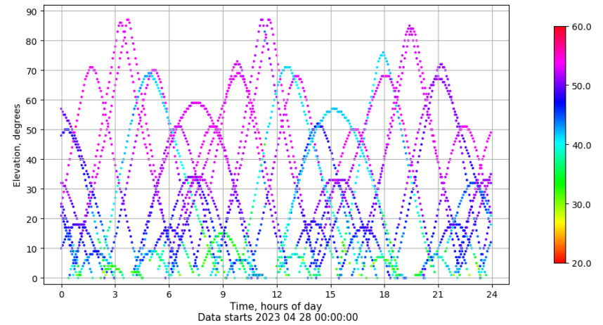
Time-elevation plot for station SALA. Signal to Noise S1C Data file SALA00ESP_R_2023118.xtr
