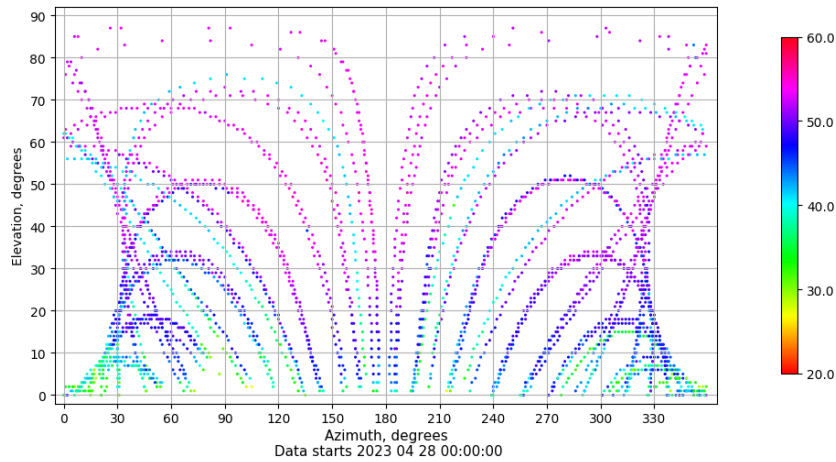
Azimuth-elevation plot for station SALA. Signal to Noise S1C Data file SALA00ESP_R_2023118.xtr
