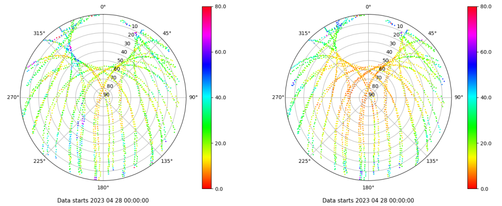
Skyplot for station SALA. Parameter M1C Data file SALA00ESP_R_2023118.xtr Skyplot for station SALA. Parameter M2P Data file SALA00ESP_R_2023118.xtr
