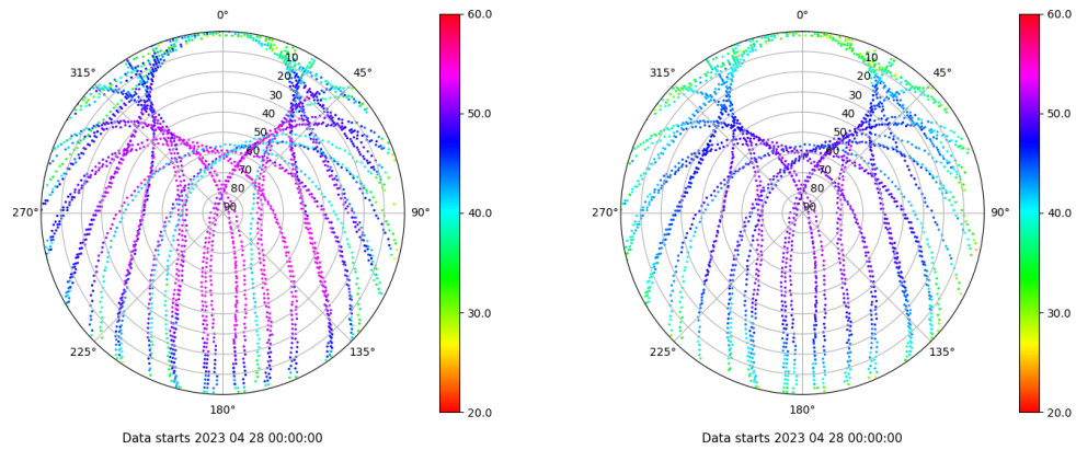
Skyplot for station SALA. Signal to Noise S1C Data file SALA00ESP_R_2023118.xtr Skyplot for station SALA. Signal to Noise S2P Data file SALA00ESP_R_2023118.xtr
