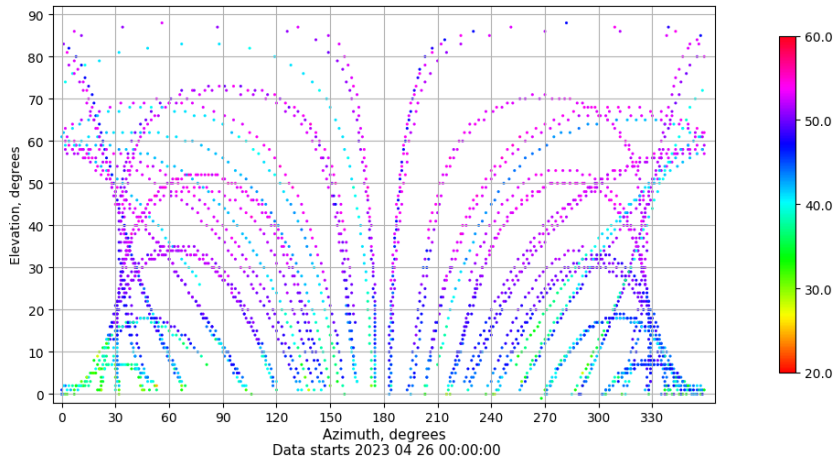
Azimuth-elevation plot for station SALA. Signal to Noise S1C Data file SALA00ESP_R_2023116.xtr
