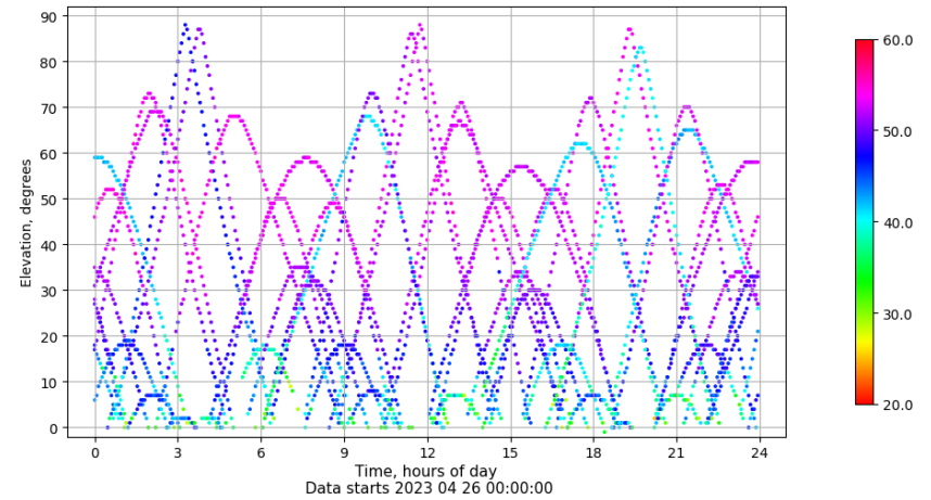
Time-elevation plot for station SALA. Signal to Noise S1C Data file SALA00ESP_R_2023116.xtr
