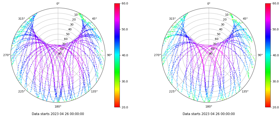
Skyplot for station SALA. Signal to Noise S1C Data file SALA00ESP_R_2023116.xtr Skyplot for station SALA. Signal to Noise S2S Data file SALA00ESP_R_2023116.xtr
