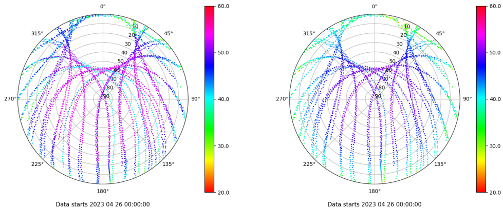
Skyplot for station SALA. Signal to Noise S1C Data file SALA00ESP_R_2023116.xtr Skyplot for station SALA. Signal to Noise S2P Data file SALA00ESP_R_2023116.xtr
