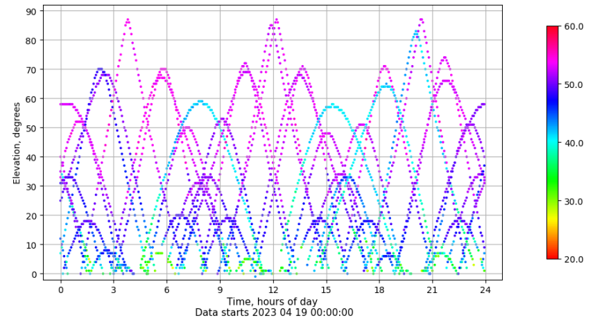
Time-elevation plot for station SALA. Signal to Noise S1C Data file SALA00ESP_R_2023109.xtr
