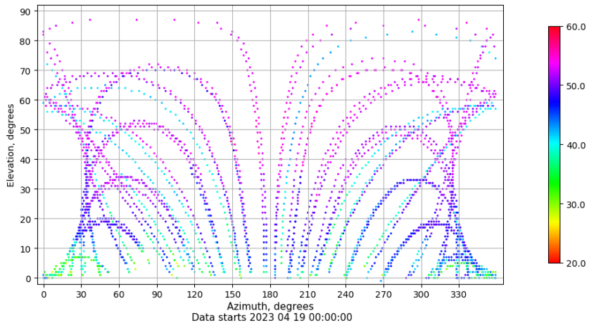
Azimuth-elevation plot for station SALA. Signal to Noise S1C Data file SALA00ESP_R_2023109.xtr
