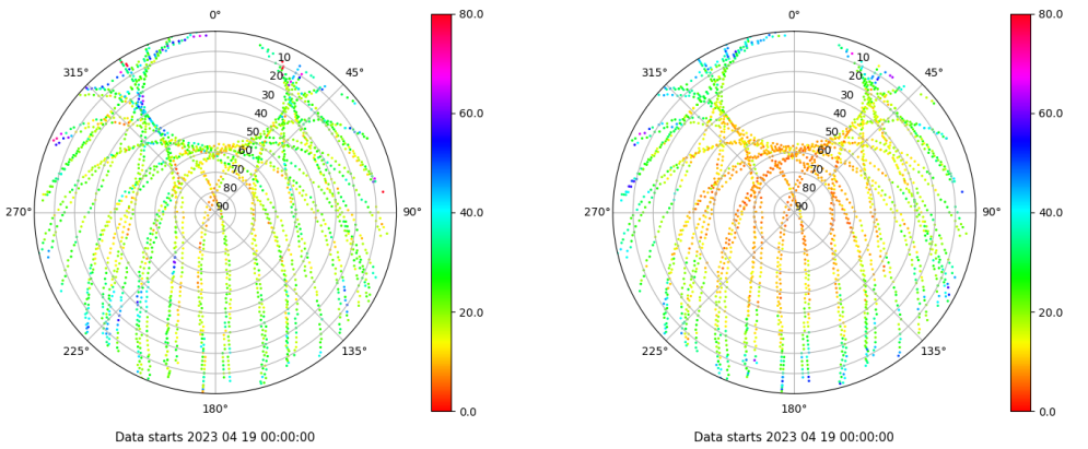
Skyplot for station SALA. Parameter M1C Data file SALA00ESP_R_2023109.xtr Skyplot for station SALA. Parameter M2P Data file SALA00ESP_R_2023109.xtr
