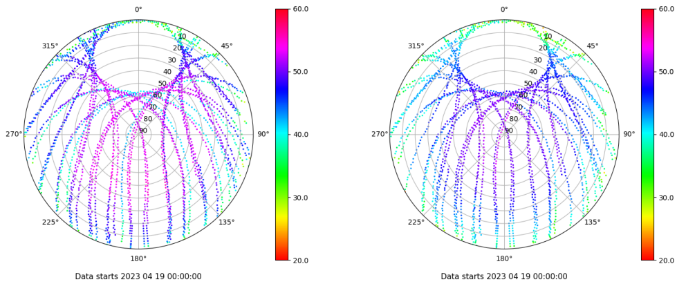
Skyplot for station SALA. Signal to Noise S1C Data file SALA00ESP_R_2023109.xtr Skyplot for station SALA. Signal to Noise S2P Data file SALA00ESP_R_2023109.xtr
