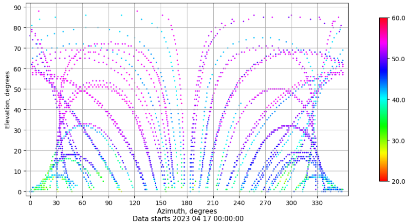
Azimuth-elevation plot for station SALA. Signal to Noise S1C Data file SALA00ESP_R_2023107.xtr
