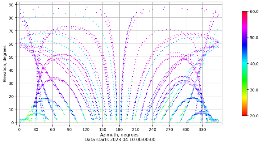
Azimuth-elevation plot for station SALA. Signal to Noise S1C Data file SALA00ESP_R_2023100.xtr
