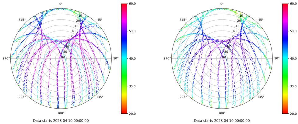
Skyplot for station SALA. Signal to Noise S1C Data file SALA00ESP_R_2023100.xtr Skyplot for station SALA. Signal to Noise S2P Data file SALA00ESP_R_2023100.xtr
