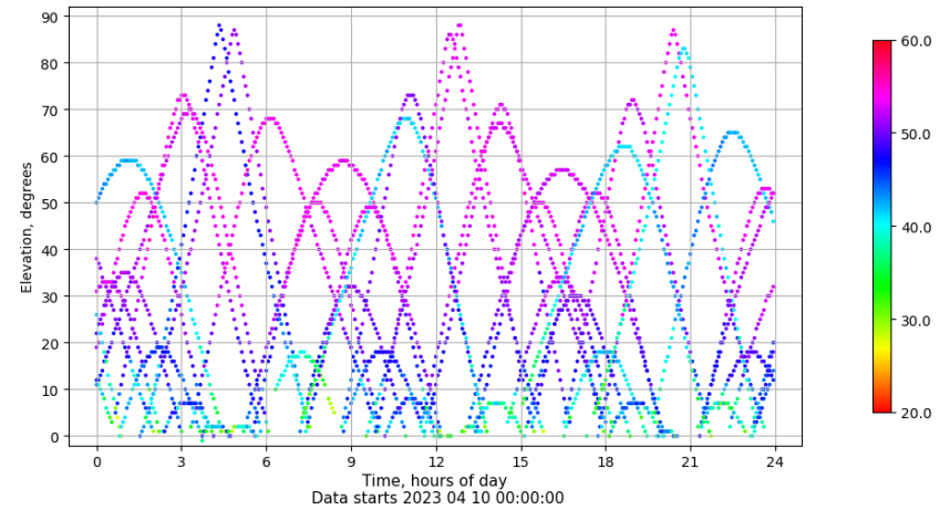
Time-elevation plot for station SALA. Signal to Noise S1C Data file SALA00ESP_R_2023100.xtr
