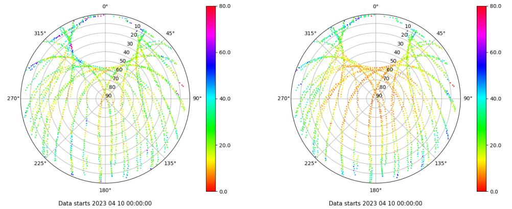
Skyplot for station SALA. Parameter M1C Data file SALA00ESP_R_2023100.xtr Skyplot for station SALA. Parameter M2P Data file SALA00ESP_R_2023100.xtr
