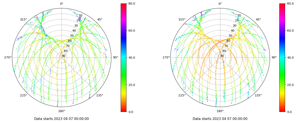
Skyplot for station SALA. Parameter M1C Data file SALA00ESP_R_2023097.xtr Skyplot for station SALA. Parameter M2P Data file SALA00ESP_R_2023097.xtr
