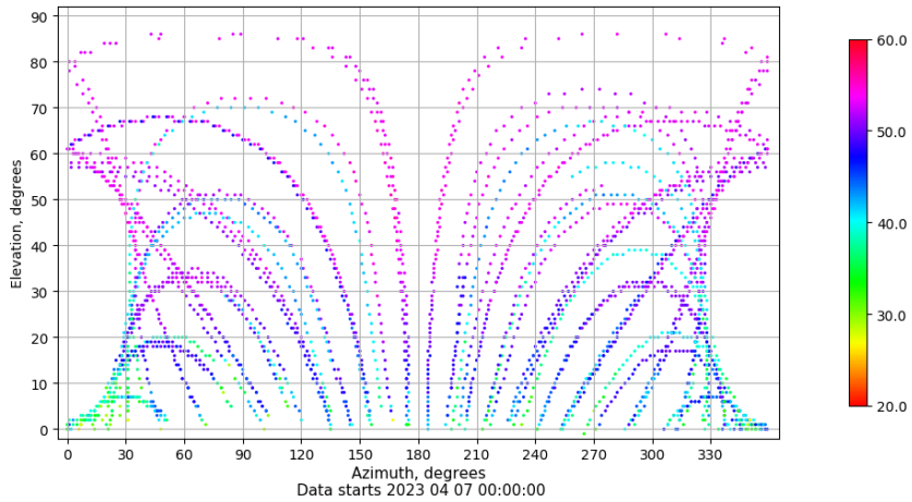
Azimuth-elevation plot for station SALA. Signal to Noise S1C Data file SALA00ESP_R_2023097.xtr
