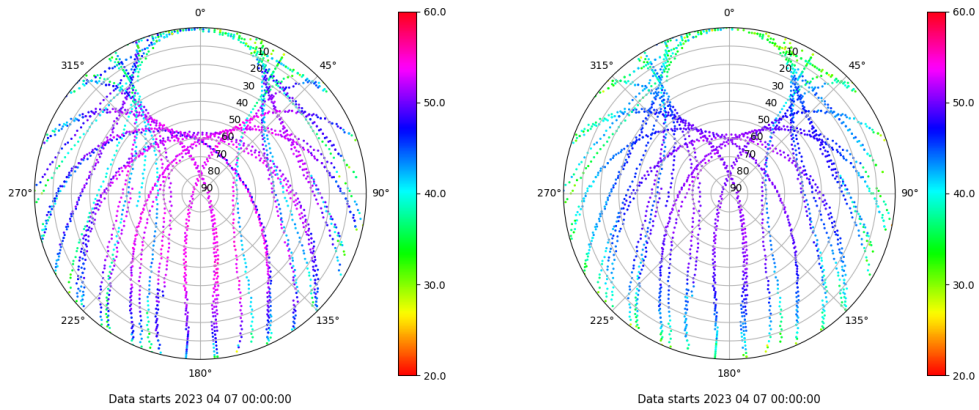
Skyplot for station SALA. Signal to Noise S1C Data file SALA00ESP_R_2023097.xtr Skyplot for station SALA. Signal to Noise S2P Data file SALA00ESP_R_2023097.xtr
