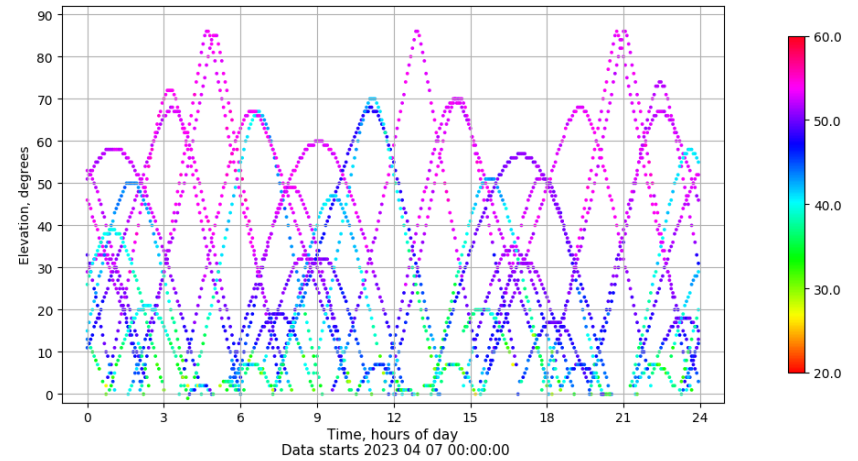
Time-elevation plot for station SALA. Signal to Noise S1C Data file SALA00ESP_R_2023097.xtr
