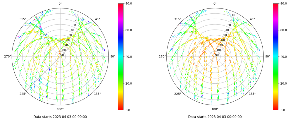
Skyplot for station SALA. Parameter M1C Data file SALA00ESP_R_2023093.xtr Skyplot for station SALA. Parameter M2P Data file SALA00ESP_R_2023093.xtr
