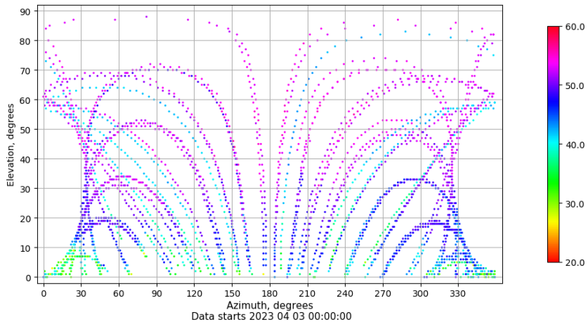
Azimuth-elevation plot for station SALA. Signal to Noise S1C Data file SALA00ESP_R_2023093.xtr
