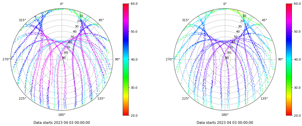
Skyplot for station SALA. Signal to Noise S1C Data file SALA00ESP_R_2023093.xtr Skyplot for station SALA. Signal to Noise S2P Data file SALA00ESP_R_2023093.xtr
