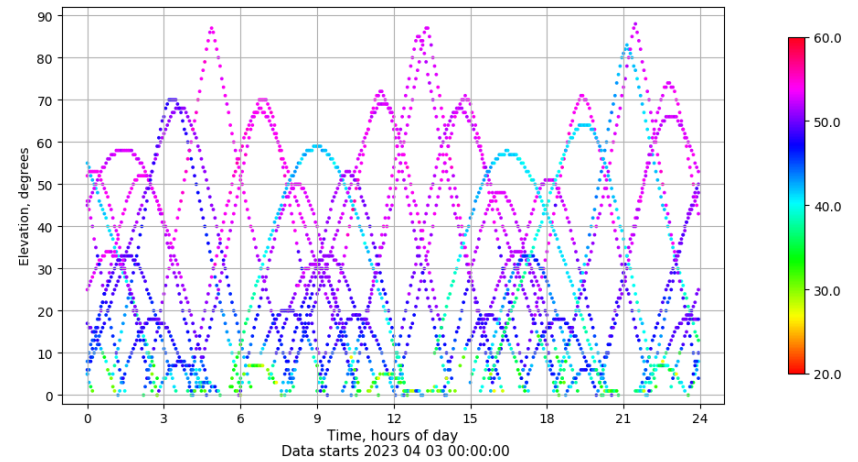
Time-elevation plot for station SALA. Signal to Noise S1C Data file SALA00ESP_R_2023093.xtr
