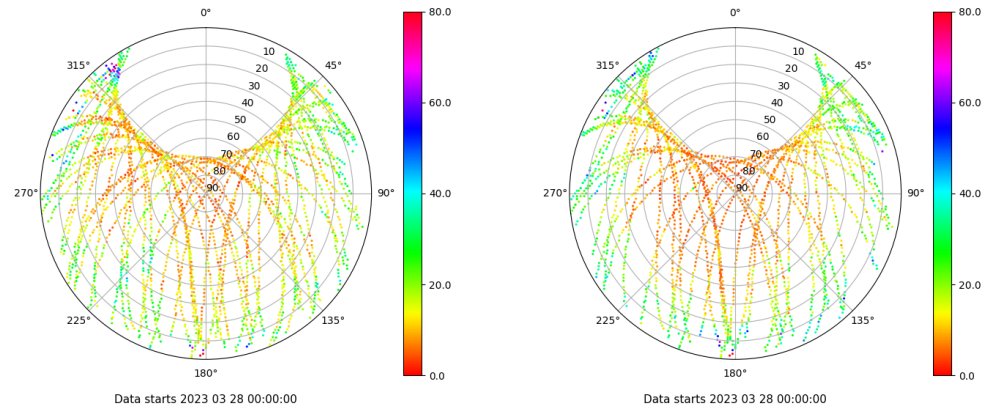
Skyplot for station SALA. Parameter M1C Data file SALA00ESP_R_2023087.xtr Skyplot for station SALA. Parameter M2S Data file SALA00ESP_R_2023087.xtr
