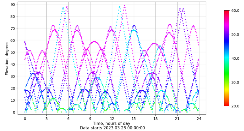
Time-elevation plot for station SALA. Signal to Noise S1C Data file SALA00ESP_R_2023087.xtr
