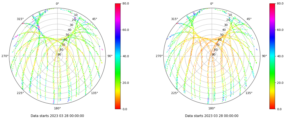
Skyplot for station SALA. Parameter M1C Data file SALA00ESP_R_2023087.xtr Skyplot for station SALA. Parameter M2P Data file SALA00ESP_R_2023087.xtr
