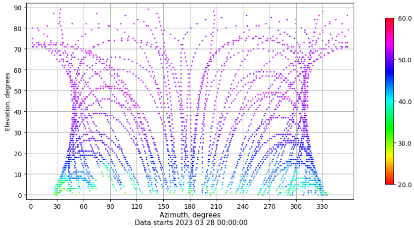
Azimuth-elevation plot for station SALA. Signal to Noise S1C Data file SALA00ESP_R_2023087.xtr
