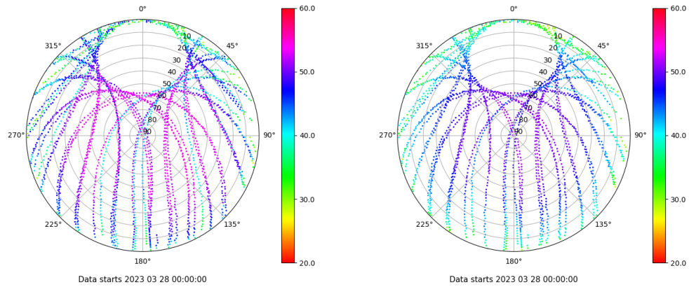
Skyplot for station SALA. Signal to Noise S1C Data file SALA00ESP_R_2023087.xtr Skyplot for station SALA. Signal to Noise S2P Data file SALA00ESP_R_2023087.xtr
