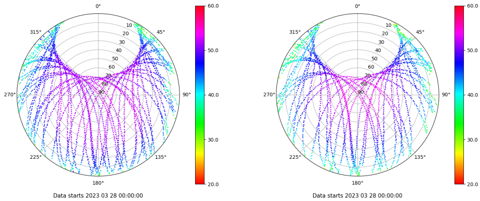
Skyplot for station SALA. Signal to Noise S1C Data file SALA00ESP_R_2023087.xtr Skyplot for station SALA. Signal to Noise S2S Data file SALA00ESP_R_2023087.xtr
