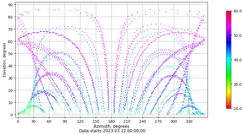
Azimuth-elevation plot for station SALA. Signal to Noise S1C Data file SALA00ESP_R_2023081.xtr
