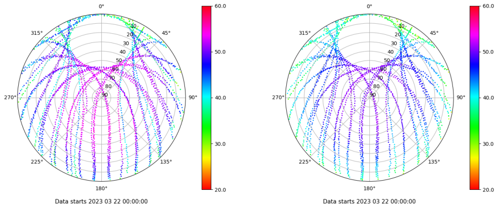
Skyplot for station SALA. Signal to Noise S1C Data file SALA00ESP_R_2023081.xtr Skyplot for station SALA. Signal to Noise S2P Data file SALA00ESP_R_2023081.xtr
