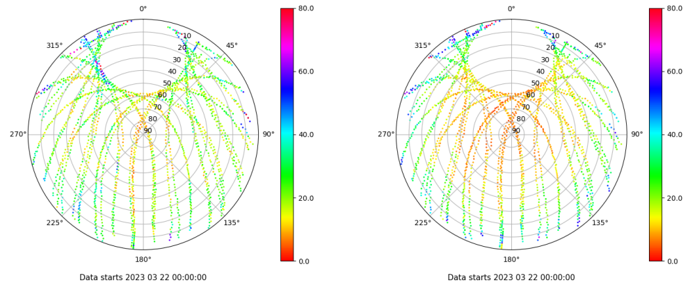
Skyplot for station SALA. Parameter M1C Data file SALA00ESP_R_2023081.xtr Skyplot for station SALA. Parameter M2P Data file SALA00ESP_R_2023081.xtr
