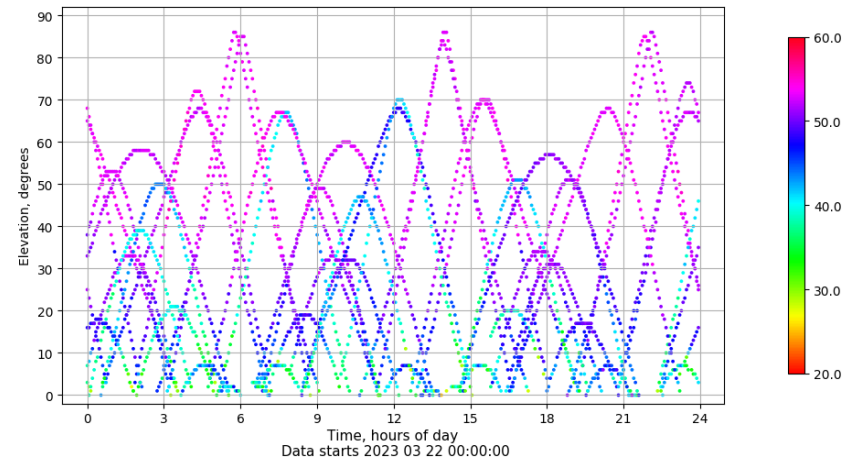
Time-elevation plot for station SALA. Signal to Noise S1C Data file SALA00ESP_R_2023081.xtr
