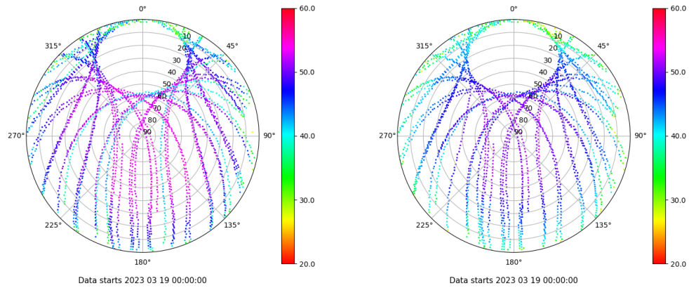
Skyplot for station SALA. Signal to Noise S1C Data file SALA00ESP_R_2023078.xtr Skyplot for station SALA. Signal to Noise S2P Data file SALA00ESP_R_2023078.xtr
