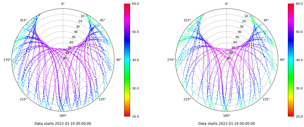
Skyplot for station SALA. Signal to Noise S1C Data file SALA00ESP_R_2023078.xtr Skyplot for station SALA. Signal to Noise S2S Data file SALA00ESP_R_2023078.xtr
