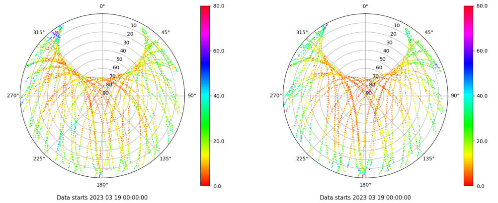
Skyplot for station SALA. Parameter M1C Data file SALA00ESP_R_2023078.xtr Skyplot for station SALA. Parameter M2S Data file SALA00ESP_R_2023078.xtr
