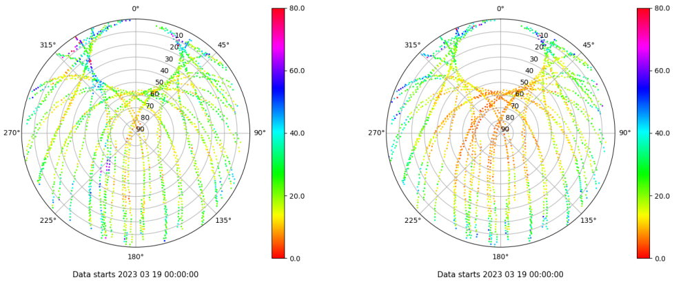
Skyplot for station SALA. Parameter M1C Data file SALA00ESP_R_2023078.xtr Skyplot for station SALA. Parameter M2P Data file SALA00ESP_R_2023078.xtr
