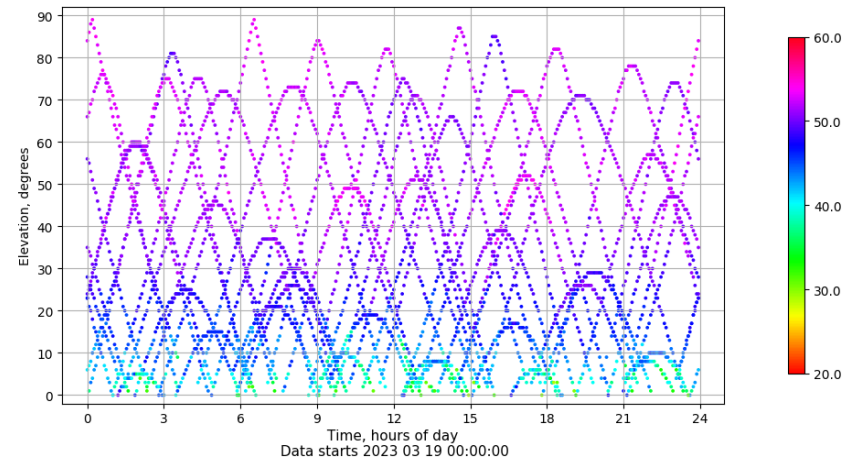
Time-elevation plot for station SALA. Signal to Noise S1C Data file SALA00ESP_R_2023078.xtr
