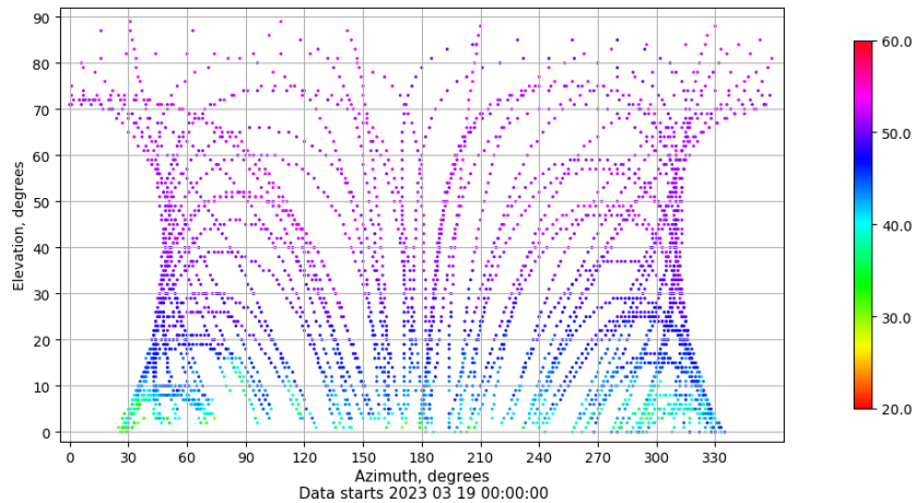
Azimuth-elevation plot for station SALA. Signal to Noise S1C Data file SALA00ESP_R_2023078.xtr
