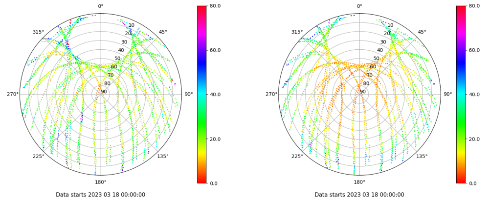
Skyplot for station SALA. Parameter M1C Data file SALA00ESP_R_2023077.xtr Skyplot for station SALA. Parameter M2P Data file SALA00ESP_R_2023077.xtr
