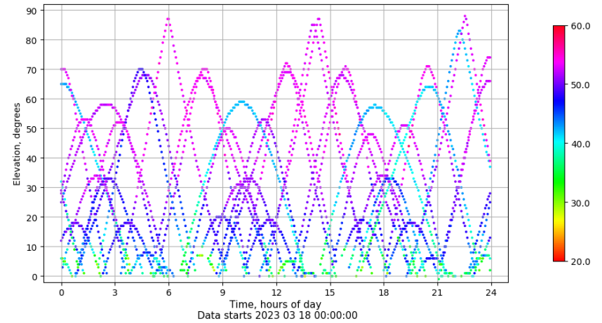
Time-elevation plot for station SALA. Signal to Noise S1C Data file SALA00ESP_R_2023077.xtr
