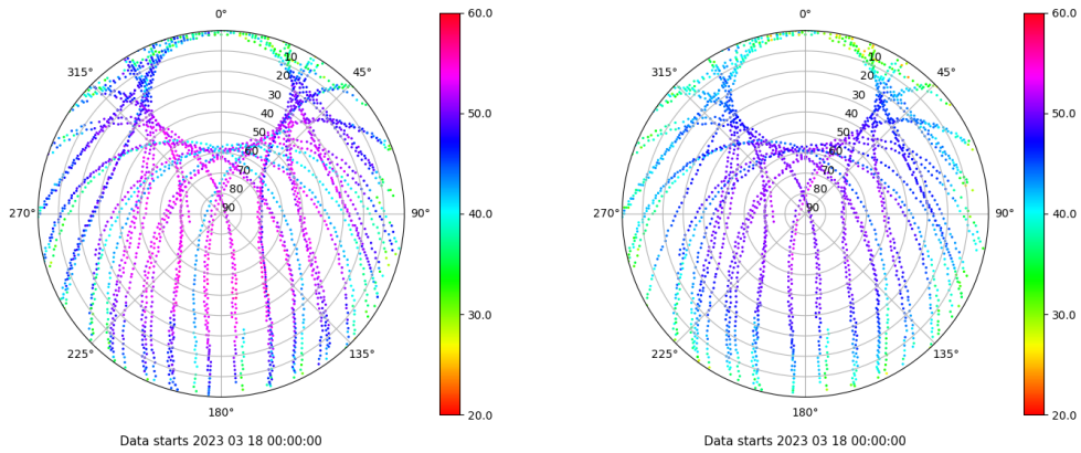
Skyplot for station SALA. Signal to Noise S1C Data file SALA00ESP_R_2023077.xtr Skyplot for station SALA. Signal to Noise S2P Data file SALA00ESP_R_2023077.xtr
