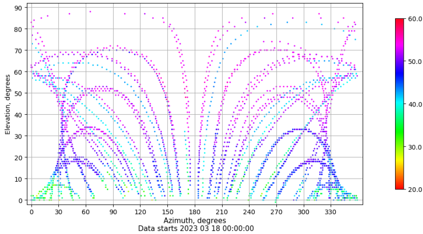
Azimuth-elevation plot for station SALA. Signal to Noise S1C Data file SALA00ESP_R_2023077.xtr
