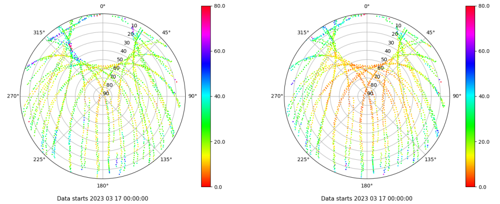
Skyplot for station SALA. Parameter M1C Data file SALA00ESP_R_2023076.xtr Skyplot for station SALA. Parameter M2P Data file SALA00ESP_R_2023076.xtr
