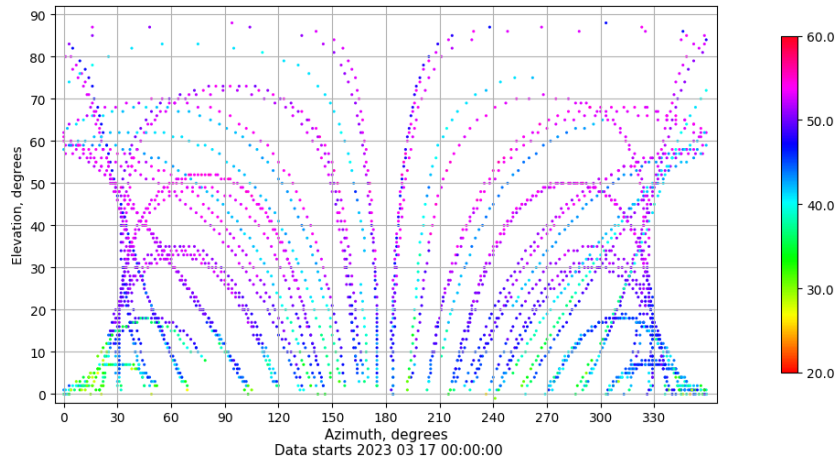
Azimuth-elevation plot for station SALA. Signal to Noise S1C Data file SALA00ESP_R_2023076.xtr
