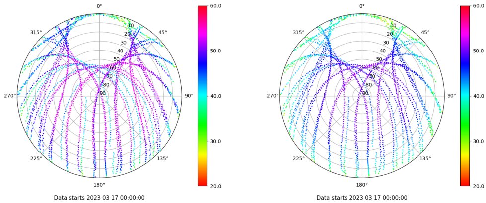
Skyplot for station SALA. Signal to Noise S1C Data file SALA00ESP_R_2023076.xtr Skyplot for station SALA. Signal to Noise S2P Data file SALA00ESP_R_2023076.xtr
