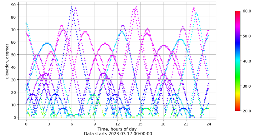
Time-elevation plot for station SALA. Signal to Noise S1C Data file SALA00ESP_R_2023076.xtr
