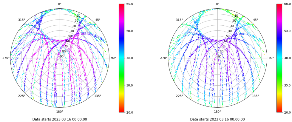
Skyplot for station SALA. Signal to Noise S1C Data file SALA00ESP_R_2023075.xtr Skyplot for station SALA. Signal to Noise S2P Data file SALA00ESP_R_2023075.xtr
