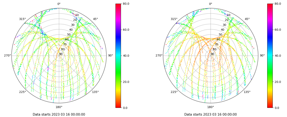
Skyplot for station SALA. Parameter M1C Data file SALA00ESP_R_2023075.xtr Skyplot for station SALA. Parameter M2P Data file SALA00ESP_R_2023075.xtr
