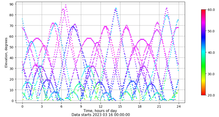
Time-elevation plot for station SALA. Signal to Noise S1C Data file SALA00ESP_R_2023075.xtr
