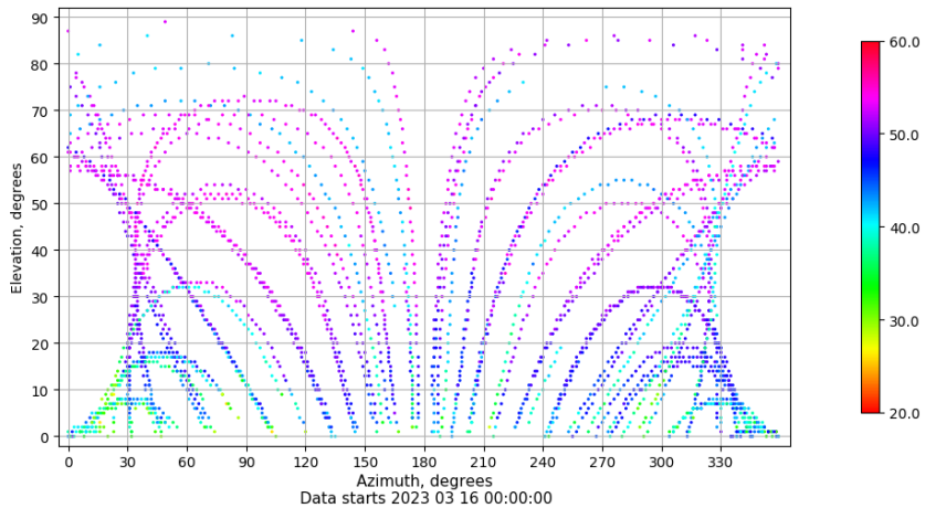
Azimuth-elevation plot for station SALA. Signal to Noise S1C Data file SALA00ESP_R_2023075.xtr
