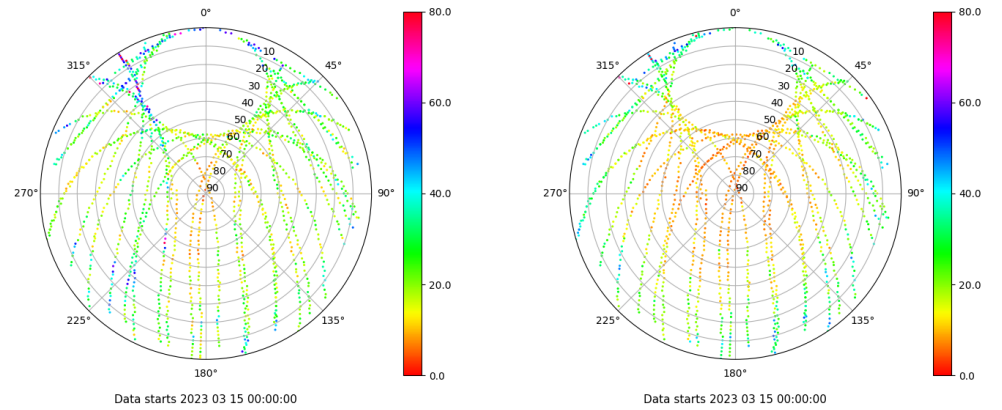
Skyplot for station SALA. Parameter M1C Data file SALA00ESP_R_2023074.xtr Skyplot for station SALA. Parameter M2P Data file SALA00ESP_R_2023074.xtr
