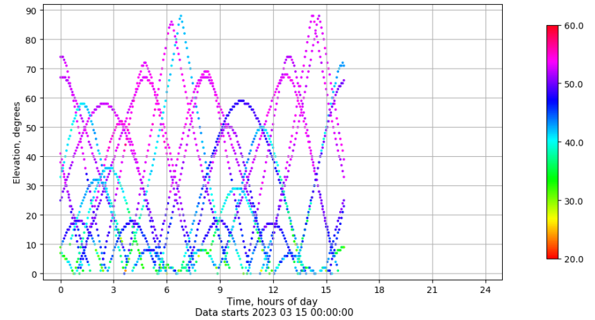
Time-elevation plot for station SALA. Signal to Noise S1C Data file SALA00ESP_R_2023074.xtr
