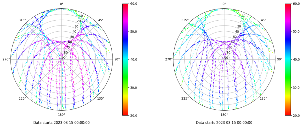
Skyplot for station SALA. Signal to Noise S1C Data file SALA00ESP_R_2023074.xtr Skyplot for station SALA. Signal to Noise S2P Data file SALA00ESP_R_2023074.xtr
