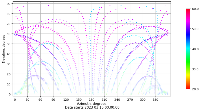
Azimuth-elevation plot for station SALA. Signal to Noise S1C Data file SALA00ESP_R_2023074.xtr
